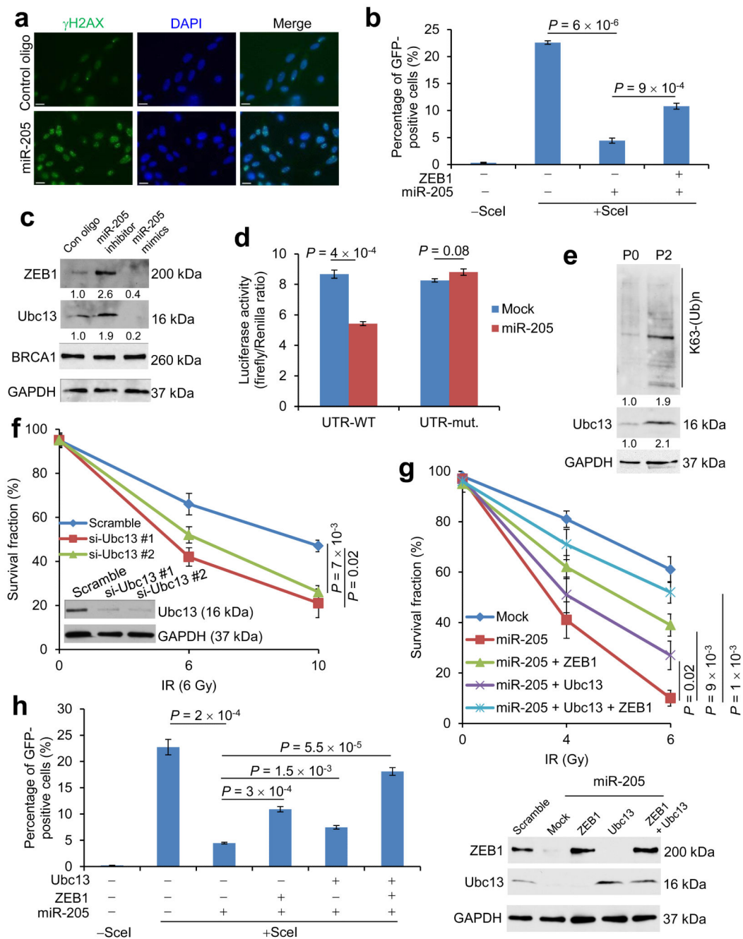
Figure 3. miR-205 regulates DNA damage repair and radiosensitivity through ZEB1 and Ubc13 (a) \gamma H2AX and DAPI staining of SUM159-P2 cells transfected with miR-205 or scramble control oligonucleotides, 24 hours after 6-Gy IR. Scale bar: 20 \mu m. (b) HR repair assays of U2OS_DR-GFP cells transfected with miR-205 alone or in combination with ZEB1. n = 3 wells per group. (c) Immunoblotting of ZEB1, Ubc13, BRCA1 and GAPDH in SUM159-P0 cells transfected with miR-205 mimics or the miR-205 inhibitor.
