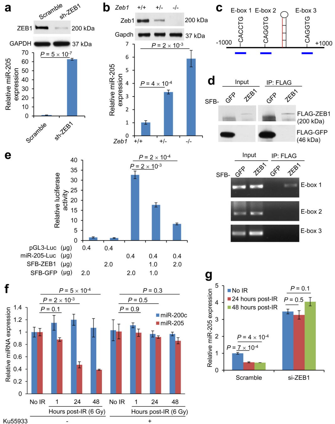
Figure 4. Radiation downregulates miR-205 expression through ZEB1 and ATM
