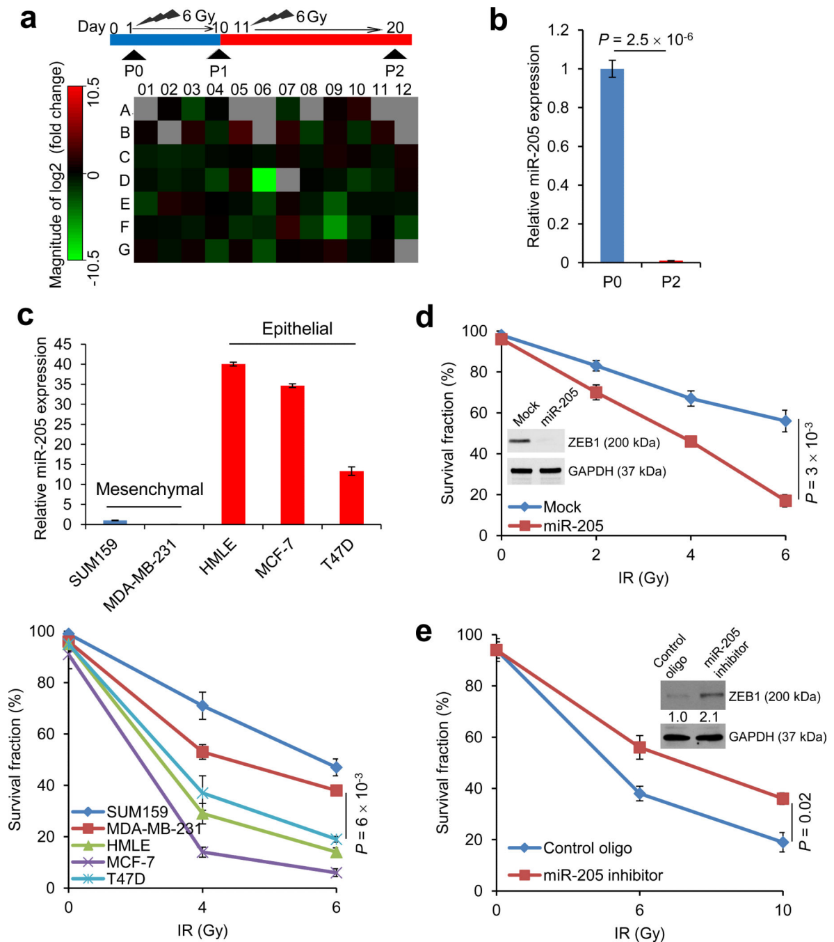
Figure 1. miR-205 increases radiosensitivity and is downregulated in radioresistant breast cancer cells
