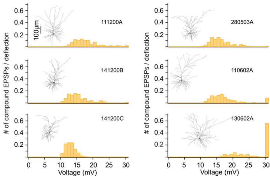
Figure 7. Response variability to whisker deflection due to difference in morphology of L2/3 pyramidal cells. The dendritic arbor of modeled cells is depicted in the inset of each panel and the corresponding distribution of composite PSPs amplitude following whisker deflection predicted by the model is shown in orange. Modeled synapses were activated based on the average PSTHs measured in vivo from both L2/3 and L4 neurons (red and yellow PSTHs in Fig. 5a bottom). In all 6 neurons modeled, the same specific R_m , C_m , and R_i values were used with identical number of synapses activated and same statistics for their spatial distribution over the dendritic tree (see Materials and Methods section). The only difference between these cases is in the morphology of the modeled postsynaptic L2/3 pyramidal cells. Details are provided in Table 2.
