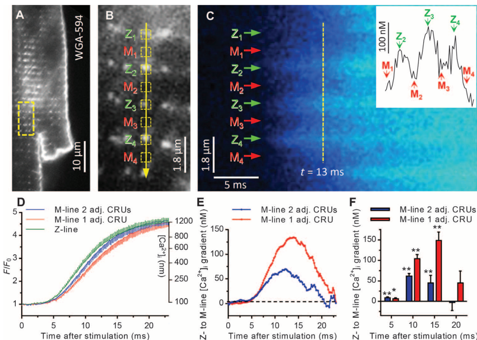
Fig. 2. Sarcomeric calcium gradients in ventricular myocytes. (A) Single cardiac myocyte labeled with a lipophilic wheat germ agglutinin conjugated to Alexa Fluor 594 to identify t-tubule CRUs. Yellow box indicates area expanded in (B). (B) Line of yellow arrow represents confocal line scan across several CRUs. Only confirmed CRUs and their adjacent M-lines were scanned. Yellow boxes represent 5-pixel regions of interest (ROIs) (500 nm) over the Z- and M-line regions. (C) Rising phase of the calcium transient ( [Ca^{2+}]_i ) from scanned region depicted in (B) immediately after stimulation of ventricular myocyte loaded with fluorescent calcium indicator. Certain M-lines are flanked by two adjacent CRUs that release calcium immediately upon stimulation (for example, M_2 and M_3 ), whereas others are adjacent to only one CRU that is triggered (for example, M_1 and M_4 ). The inset depicts the spatial profile of [Ca^{2+}]_i 13 ms after stimulation (vertical yellow line). (D) Average [Ca^{2+}]_i transient \pm error bars (SEM) rising phase time course from 59 Z-line CRUs (green, n = 12 cells) and their adjacent (adj.) M-lines when flanked by two triggered CRUs (blue, n = 59 sites, 12 cells) and a single triggered CRU (red, n = 53 sites, 12 cells). (E) Z- to M-line [Ca^{2+}]_i gradient calculated by subtracting M-line from Z-line traces in (D). (F) Z- to M-line [Ca^{2+}]_i gradient \pm SEM 5, 10, 15, and 20 ms after stimulation in sarcomeres. *P < 0.01 , **P < 0.001 , one-sample t test.
