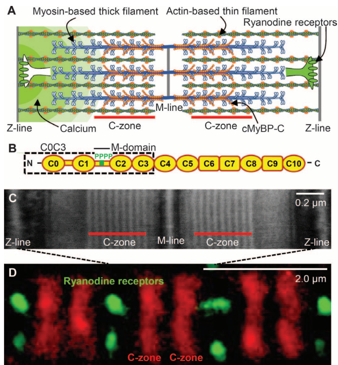
Fig. 1. Sarcomeric organization and MyBP-C. (A) Cardiac muscle sarcomere with interdigitating thick and thin filaments. MyBP-C localized to the C-zone, whereas the ryanodine receptors are localized in puncta (CRUs) along the Z-lines, forming the boundaries of each sarcomere. (B) Schematic diagram of cardiac MyBP-C's Ig-like (oval) and fibronectin-like (rectangular) domains with four phosphorylation sites (P) in the M-domain and COC3 fragment (dashed box) used in the 3D EM and in vitro motility experiments. (C) Negatively stained EM image of a sarcomere within a mouse ventricular myocyte labeled with antibodies to MyBP-C. (D) Two-color dSTORM super-resolution image of sarcomeres as in (C), labeled with Alexa Fluor-conjugated antibodies to MyBP-C and ryanodine receptors.
