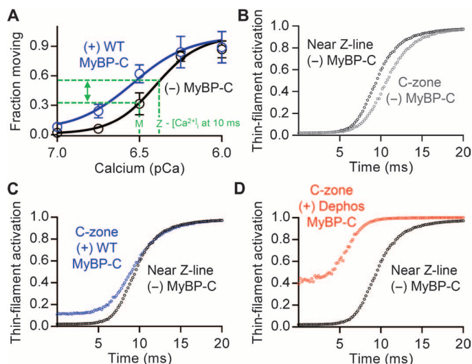
Fig. 4. Effect of [Ca^{2+}]_i on thin filament activation in the absence of MyBP-C near the Z-line and presence of MyBP-C within the C-zone. (A) Fraction of thin filaments moving \pm SEM–pCa plots within the Z- and M-line regions of the sarcomere in the (black) absence and (blue) presence of wild-type (WT) MyBP-C. [Ca^{2+}]_i in the Z- and M-line regions 10 ms after cardiac excitation indicated (green dashed lines). (B to D) Model generated estimates of thin filament activation after calcium release. Thin filament activation–time plot generated for regions of the thin filaments near the Z-lines (black) and within the C-zone, near the center of the sarcomere. (B) Model assumes that the C-zone lacks MyBP-C and thus predicts that thin filament activation in the C-zone (gray) would lag behind the Z-line. (C) Model assumes normally phosphorylated wild-type MyBP-C in C-zone (blue) and predicts that C-zone activation level would no longer lag behind the Z-line. (D) Model assumes dephosphorylated MyBP-C within C-zone (red), resulting in a sensitized C-zone that would contribute to significant activation even during relaxation.
