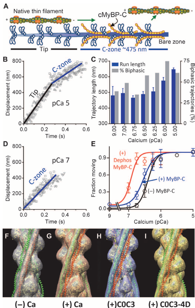
Fig. 3. The effects of MyBP-C on native thin filament activation. (A) Illustration of a thin-filament shard traveling over one-half of a native thick filament, as in TIRFM experiments. (B) Displacement-time plots for five thin filaments on wild-type thick filaments at pCa 5 demonstrating two phases of velocity (black, fast; blue, slow). (C) Trajectory length \pm SEM-pCa and percent trajectories with biphasic velocities (as in B)–pCa histograms for thin filaments on wild-type thick filaments. (D) As in (B) for five filaments at pCa 7 demonstrating movement only within the thick filament C-zone. (E) Fraction of thin filaments moving \pm SEM-pCa plots for thin filament motion in the absence of (black) and presence of wild-type (blue) and \lambda -phosphatase-treated MyBP-C (red). Data fitted with sigmoidal dose-response curves with differing pCa 50 ( P < 0.001 , extra sum-squares F test). Dephos, dephosphorylated with \lambda -phosphatase. (F and G) 3D structure of native thin filaments with tropomyosin (Tm) in the (F) “blocked” position in the absence of and (G) “closed” position in the presence of calcium. Atomic structures of actin with Tm in the “blocked” position (red) and “closed” position (green) were fitted to each 3D structure. (H and I) 3D structure of native thin filaments decorated with MyBP-C N-terminal fragments in the absence of calcium. Position of tropomyosin with addition of (H) C0C3 and (I) phosphomimetic C0C3-4D fragments. The 3D structure fitted with atomic structures showed Tm’s movement in thin filament decorated with C0C3 from “blocked” to “closed” position. In contrast, the fitted structures for the thin filament decorated with C0C3-4D showed only partial movement of Tm toward the “closed” position.
