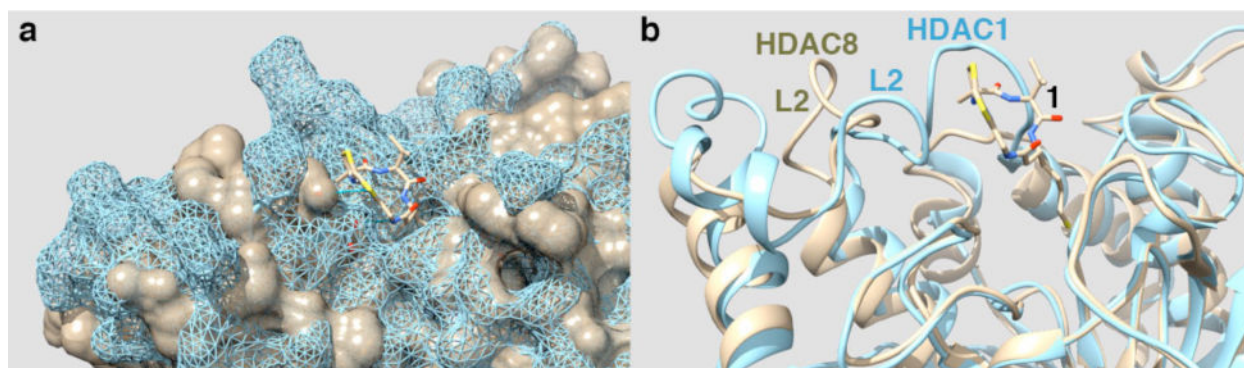
Figure 6. (a) Surface representation of the HDAC8-1 complex (brown) and HDAC1 (blue mesh). (b) Cartoon representation of the superposition in (a), with the position of the flexible loop L2 in HDAC1 and HDAC8 indicated.
