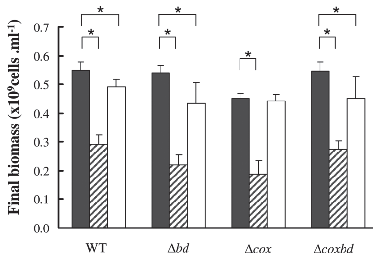
Fig 4. Biomass formation under various culturing conditions. Final biomass for the four DvH strains cultured under anaerobic conditions only (black bars), with constant 0.02% O 2 gas mixture sparging (striped bars) and after growth resumption (open bars). Data are mean values of five independent experiments + SD. Statistical analysis using t-test was used to compare means. Significant differences (p < 0.05) are mentioned by an asterisk.
