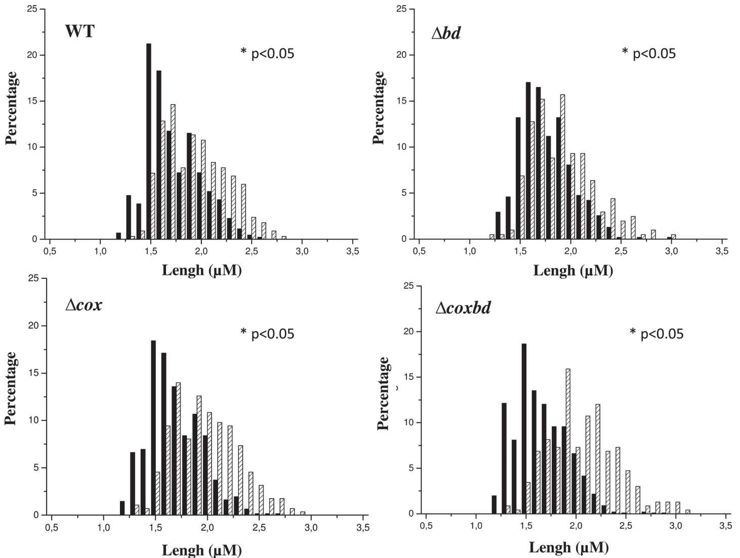
Fig 2. Variability in the cell length of the various DvH strains. Comparison of the distribution of the cell length in cultures under anaerobic conditions (black bars) and with constant 0.02% \text{O}_2 gas mixture sparging (striped bars). The average cell length was determined from two independent cultures (>200 cells were counted in each experiment). Statistical analysis using One-way ANOVA were performed to reveal significant differences between distributions ( p < 0.05 ), which were mentioned by an asterisk.
