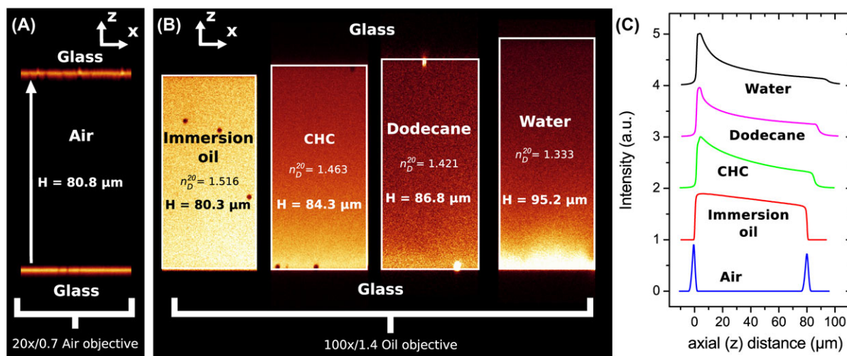
Fig. 2. Axial distances measured with confocal microscopy. (A) The empty calibration cell with H = 80.990 \pm 0.008 \mu\text{m} was measured in confocal reflection mode (Leica SP2) with a 20x/0.7 air-objective (Leica), which resulted in H = 80.8 \pm 0.3 \mu\text{m} . (B) The cell filled with immersion oil, pyromethene dye and poly(methyl methacrylate) (PMMA) tracer particles (left). The sample was imaged with an 100x/1.4 oil objective (Leica) and a similar height was measured ( H = 80.3 \mu\text{m} ). However, when the cell was re-filled with solvents that had a RI mismatch with the oil-objective, deviating axial-distances were found, as indicated in the figure. (C) Intensity profiles along the axial ( z ) direction show the increase in (apparent) axial distance as well as decrease of intensity deeper in the sample. The profiles were normalized and shifted for better visualization.
