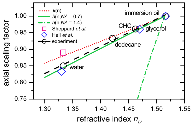
Fig. 3. Axial scaling factors as a function of the sample refractive index n_D . Our measurements are indicated with black open circles, which were fitted with the dashed (black) line. The (green) continuous and (green) dashed-dotted lines are from the high-angle geometrical prediction of Eq. (2), for NA = 0.7 and NA = 1.4, respectively, and the (red) dotted line is from the paraxial limit of Eq. (3). The (pink) square is based on a theoretical study by Sheppard et al. (Sheppard & Török, 1997) for NA = 1.4 and the (blue) diamonds show calculations based on a study by Hell et al. for NA = 1.3 (Hell et al. , 1993), both at a wavelength around 500 nm.
