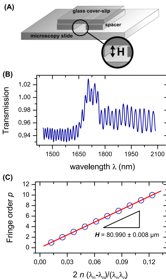
Fig. 1. Construction and measurement of a calibration cell. (A) A sample cell with height H was built with glass cover slips and a standard microscopy slide, glued together with UV-gel. (B) When the (empty) cell was placed in a Fourier Transform Infrared (FTIR) spectrometer, Fabry Perrot (FP) fringes were visible in the transmission spectrum. (C) The height of the cavity ( H = 80.990 \pm 0.008 \mu\text{m} ) was determined from the spacing between the FP fringes (Jiang et al. , 1999). The error-bars on individual points are smaller than the symbol size.
