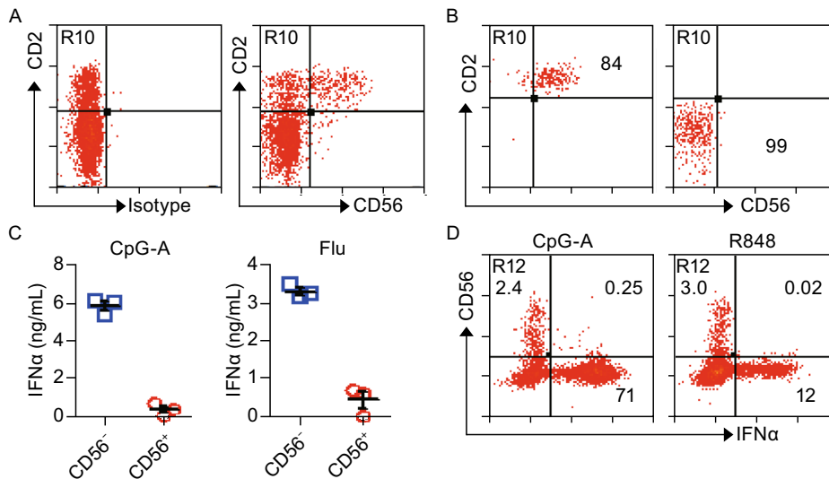
Figure 2. CD56 + DCs are functionally distinct from pDCs. (A) Human PBMC were gated on Lin - HLA-DR + CD11c - CD123 + DCs, and the gated DCs were analyzed by their CD2 and CD56 expression. (B) Lineage depleted PBMC were gated on Lin - HLA-DR + CD11c - CD123 + DCs, then CD2 + CD56 + and CD2 - CD56 - DCs were sorted by FACS. The purities of sorted cells are shown in each plot. (C) 10,000 purified CD123 + CD56 - and CD123 + CD56 + DCs were stimulated with CpG A or influenza virus (Flu) for 24 h, then interferon \alpha (IFN \alpha ) in the supernatants were analyzed by ELISA. Data summarized from 3 independent donors. (D) Lineage depleted PBMCs were stimulated with CpG A or R848 then analyzed by FACS for surface markers and IFN \alpha intracellularly. Lin - HLADR + CD11c - CD123 + cells were gated and plotted for CD56 and IFN \alpha . The numbers in each quadrant represent percentage of total gated cells. One out of four independent experiments is shown.
