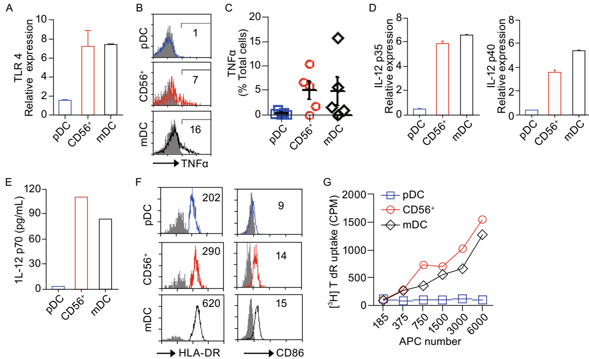
Figure 4. CD56 + DCs functionally resemble mDCs. (A) The expression of TLR4 was quantified by RT-PCR with purified DCs. Error bars represent standard deviation from duplicated PCR samples of the same donor. Data shown are from one representative of 3 independent donors. (B) Lineage depleted PBMC were stimulated with LPS for 6 h, then the stimulated cells were collected and stained with surface markers followed by intracellular staining of TNF \alpha . CD123 + CD56 - (pDC), CD123 + CD56 + (CD56 + ) and CD123 - CD11c + (mDC) in the Lin - HLA-DR + gate were analyzed for TNF \alpha expression. (C) Summarized data of (B) from 5 independent donors. (D) Purified DCs were stimulated with mixture of LPS, CpG and IFN \gamma for 6 h, the expression of IL-12 p35 and p40 were analyzed by RT-PCR. Data shown are representative of 3 independent experiments. (E) Purified DCs were stimulated mixture of LPS, CpG and IFN \gamma for 24 h, and the expression of IL-12 p70 were analyzed by ELISA. Data shown are representative of 2 independent experiments. (F) Expression of HLA-DR and CD86 on different blood DC subsets were analyzed by FACS. (G) Purified allogenic naive T cells were cocultured with different numbers of CD123 + CD56 - (pDC, circle), CD123 + CD56 + (CD56 + , square) and CD123 - CD11c + (mDC, triangle) DCs. After 5 days, the cocultured cells were pulsed with 1 mCi [ 3 H] thymidine for 18 h before harvest. Data shown are one representative of 4 experiments.
