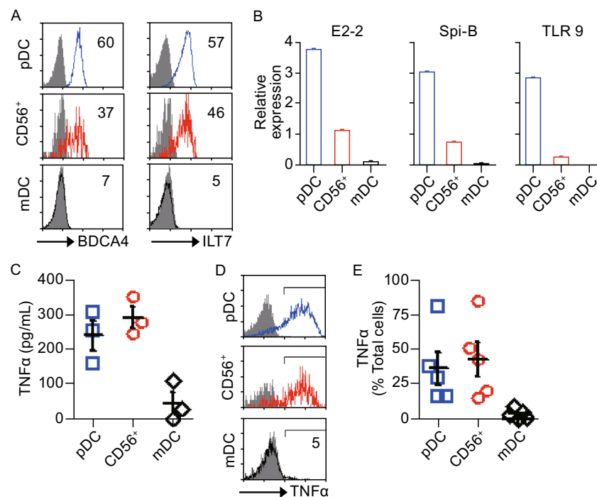
Figure 5. CD56 + DCs adopt certain characteristics attributed to pDCs. (A) The expression of BDCA4 and ILT7 in different DC subpopulations from PBMC were analyzed by FACS. Data shown are one representative of 3 donors. (B) CD123 + CD56 - (pDC), CD123 + CD56 + (CD56 + ) and CD123 - CD11C + (mDC) were purified from PBMC, E2-2, Spi-B and TLR9 expression in those three DC populations were analyzed by RT-PCR. Error bars represent standard deviation from duplicated PCR samples of same donor. Data shown are one representative of 3 donors. (C) Purified DCs were stimulated with CpG B for 24 h, and the expression of TNF \alpha were analyzed by ELISA. Data shown are summarized from 3 independent experiments. (D) Lineage depleted PBMCs were stimulated with CpG B for 6 h, then stimulated cells were collected and stained with Lin, HLA-DR, CD123, CD11C and CD56 followed by intracellular staining of TNF \alpha . The Lin - HLA-DR + cells were divided into CD123 + CD56 - (pDC), CD123 + CD56 + (CD56 + ) and CD123 - CD11C + (mDC) subsets, TNF \alpha expression in each DC subset were analyzed. (E) Summarized data of (D) from 5 independent donors.
