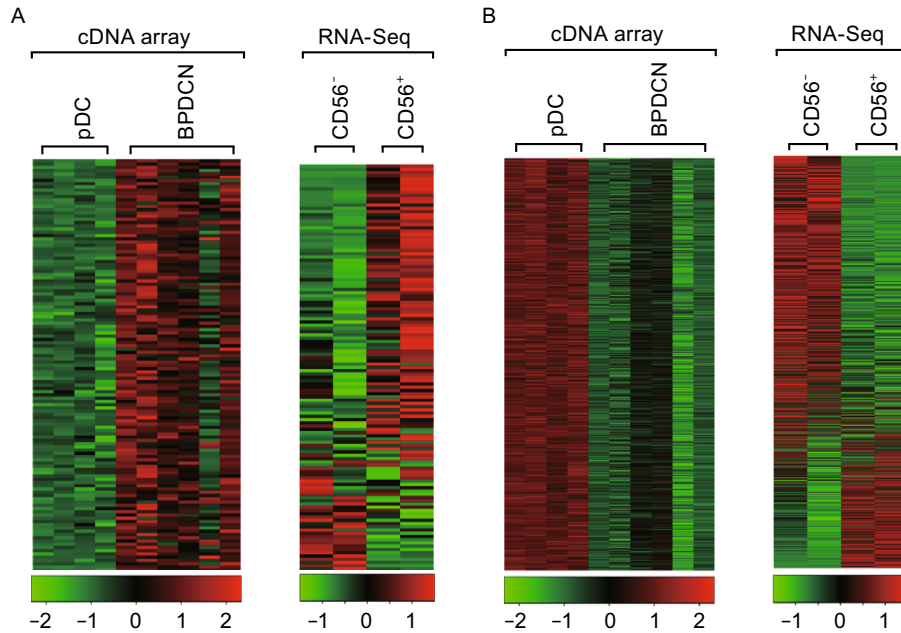
Figure 6. Global gene expression of BPDCN, pDCs and CD56 + DCs. (A) Heat map of 127 genes highly expressed in BPDCN comparing with pDCs by cDNA array (left panel) and their expressions in CD56 + DCs relative to CD56 - pDCs by RNA-Seq (right panel). (B) Heat map of 1143 genes highly expressed in pDCs comparing with BPDCN by cDNA array (left panel) and their expressions in CD56 + DCs relative to CD56 - pDCs by RNA-Seq (right panel).
