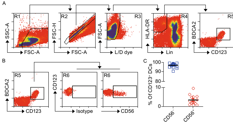
Figure 1. CD56 + DCs in human blood. (A) Human PBMC were first gated based on light scatters, and dead cells were excluded by yellow fluorescent reactive dye (L/D dye), then Lin - HLA-DR + BDCA2 + CD123 + dendritic cells (DCs) were gated for further analysis. (B) Gated Lin - HLA-DR + BDCA2 + CD123 + blood DCs were divided into two subsets by their CD56 expression. (C) Summarized data show relative abundance of CD56 - and CD56 + populations in BDCA2 + CD123 + DCs (Mean \pm SD, n = 15 ).
