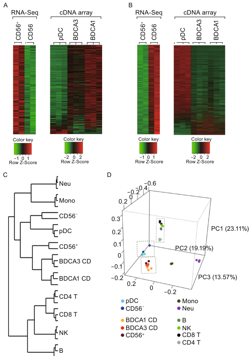
Figure 3. Comparing gene expression of CD56 + DCs and other DC subsets. (A) 648 genes expressed in CD123 + CD56 + DCs at least two fold higher than in CD123 - CD56 - DCs obtained by RNA-Seq (left panel) and their expressions in pDCs, BDCA3 mDCs and BDCA1 mDCs extracted from cDNA array data (right panel). (B) 1557 lowly expressed genes in CD123 + CD56 + relative to CD123 - CD56 - DCs (left panel) and their expressions in pDCs, BDCA3 mDCs and BDCA1 mDCs extracted from cDNA array data (right panel). (C) Clustering of CD123 + CD56 + and CD123 - CD56 - DCs with other immune cell lineages isolated from human peripheral blood based on their gene expression profiles. (D) The principal component analysis (PCA) results. Mono, monocytes; Neu, neutrophils; NK, natural killer cells.
