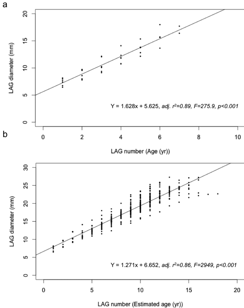
Fig. 4. The linear relationships between line of arrested growth (LAG) diameter and LAG number. The linear regression equations from these relationships were used for a) the first order correction applied to 72 bones, (humerus diameter (HD) range 17.3 to 27.5 mm, and CCL range 45 to 81 cm); and b) second order correction applied to 71 bones (HD range 20.3 to 33.6 mm, and CCL range 51 to 90 cm).
