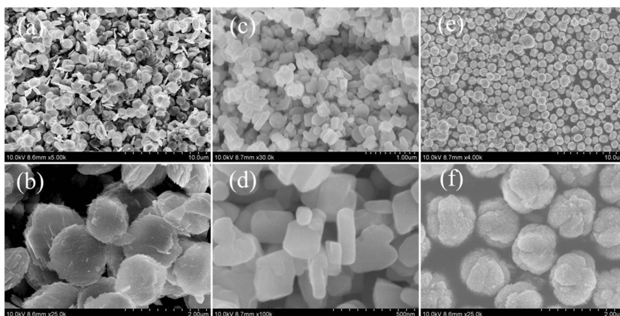
Figure 1 FE-SEM images of different structures. (a) CuO microdisks, (c) CuO nanoblocks, and (e) CuO microspheres at low magnification; (b) CuO microdisks, (d) CuO nanoblocks, and (f) CuO microspheres at high magnification.
