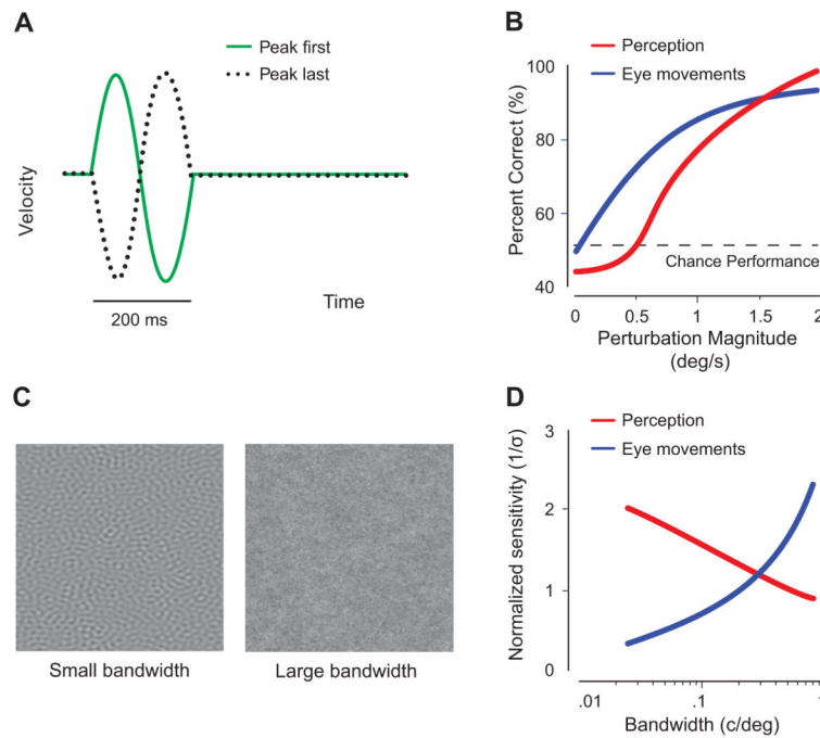
Figure 1. When eye movements and perception yield different results (A) Observers discriminated speed changes (perturbation magnitude between 0–2.5 deg/s). Stimulus speed either increased first and then decreased (peak first), or it decreased first and then increased (peak last); five speed perturbation magnitudes (in degrees per second) were tested. (B) Schematic of results from one observer. Pursuit eye movements were more sensitive to speed changes and discriminated between peak-first and peak-last changes reliably even when perception was at chance; data points below chance performance for perception, but above chance performance for pursuit. (C) OFR were elicited by large motion texture stimuli with varying spread of the spatial frequency distribution (bandwidth in cycles per degree) across trials. Eye movement velocity was compared to perceptual sensitivity in a speed discrimination task, in which mean spatial frequency and bandwidth were constant in a given trial but varied across trials. (D) Mean sensitivity results from three observers showing an opposite trend in OFR and perception. Eye movement sensitivity (inverse standard deviation of OFR velocity) increased, whereas perceptual sensitivity (inverse discrimination threshold) decreased with increasing bandwidth. [A and B adapted with the authors’ permission from Tavassoli and Ringach[44], Table 1.2; (C) and (D) adapted with the authors’ permission from Simoncini et al.[57], Table 1.3]
