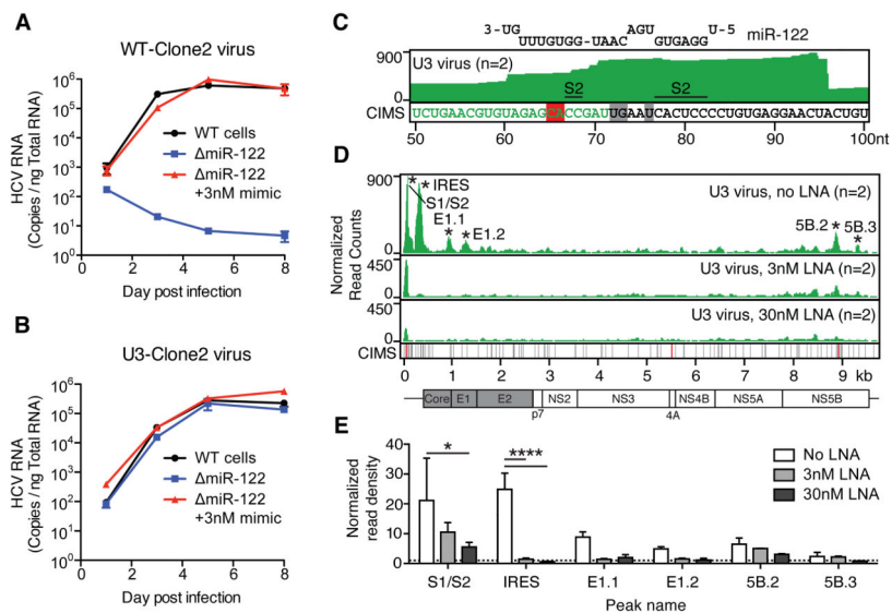
Figure 2. An HCV mutant resistant to miR-122 antagonism engages Ago and miR-122. (A–B) Timecourse qPCR measurements of WT-Clone2 virus (A) or U3-Clone2 virus (B) in WT cells or in \Delta miR-122 cells with or without 3nM miR-122 supplementation. Error bars, \pm SD. (C) Ago binding map (top track) and CIMS locations (bottom track) across the U3 virus 5'UTR corresponding to miR-122 binding at S2. Relevant CIMS deletions are shown in gray (not significant) and red (significant). U3 snoRNA sequence is shown in green. (D) Ago binding map across the U3 virus genome after treatment with increasing doses of LNA122. Significant peaks are named by location and indicated by asterisks. Bottom CIMS track shows location of all deletions (gray) and significant CIMS deletions (red) for the untreated dataset. (E) Ago binding in significant peaks from untreated U3 datasets in (D) shown as normalized read densities calculated per dataset. **** P < 0.0001 , * P < 0.05 , one-way ANOVA with bonferroni correction. Error bars, \pm SD.
