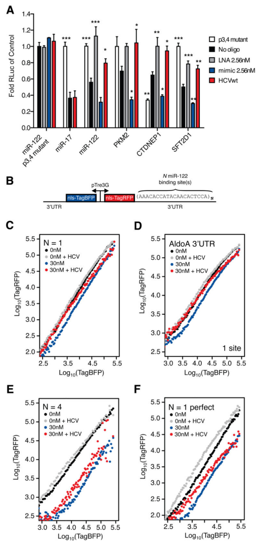
Figure 5. Validation of HCV induced de-repression of miR-122 targets in bulk and single-cell resolution. (A) Luciferase reporter measurements for synthetic miR-122, miR-17, or cellular 3'UTR target constructs. Data were normalized to “no oligo” p3,4 mutant conditions. Significance testing was performed relative to endogenous “no oligo” repression for each tested construct. Asterisks: *** P < 0.001 , ** P < 0.01 , * P < 0.05 , ANOVA with bonferroni correction. (B) Two-color fluorescent reporter containing a bidirectional Tet promoter that drives expression of blue and red fluorescent proteins (TagBFP and TagRFP). Each fluorescent protein is tagged with a nuclear localization sequence (NLS) to aid in flow cytometric analysis. The 3'UTR of TagRFP is engineered to contain N binding sites for miR-122, or full 3'UTRs of miR-122 targets. (C–F) Log-log transfer functions for N=1 (C), ALDOA 3'UTR (D), N=4 (E) or one perfectly complementary (F) miR-122 site in the presence or absence of 30nM miRNA mimic and/or HCV infection.
