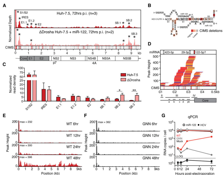
Figure 1. Argonaute binding maps on HCV RNA. (A) Mock-subtracted binding map of Ago-CLIP reads across HCV genomic RNA in WT or \Delta Drosha Huh-7.5 cells. Data were normalized to total cellular and virus read depth for comparison. Significant peaks per track are named by location and indicated by asterisks. Bottom CIMS track shows location of all deletions (gray) and statistically significant CIMS deletions (red) from the WT track. (B) Ago binding in significant peaks from WT Huh-7.5 cells in (A) shown as normalized read densities calculated per dataset. Data were normalized to background read density of non-peak regions (dashed line). Asterisks, ** P < 0.01 , * P < 0.05 , Student’s t-test. Error bars, \pm SD. (C) Schematic of a miR-122 binding model to S1 and S2 highlighting locations of CIMS deletions. (D) Zoom in view of Ago binding from WT cells in (A) across the viral IRES into the coding sequence. IRES domains (II–IV), associated stemloops (a–d) and the pseudoknot (pk) region are indicated. Upper track displays seeds for the top 50 miRNA seeds, previously proposed miR-122 binding (Pang et al., 2012) highlighted in red. (E–F) Ago binding timecourse of WT (E) and replication deficient (GNN) (F) HCV post-electroporation ( n=2 ). (G) Absolute qPCR measurements of miR-122 and HCV RNA levels at indicated time points post electroporation ( n=3 ). Replication-deficient J6/JFH1-GNN and mock controls are shown. Dashed line indicates lower limit of quantitation. Error bars, \pm SD. See also Figure S3.
