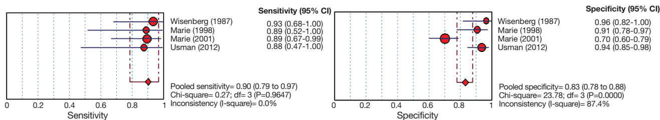
Figure 2 Forest plot of sensitivity and specificity for T2 relaxation time. CI, confidence interval.
