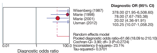
Figure 4 Forest plot of diagnostic odds ratio for T2 relaxation time. OR, odds ratio.
