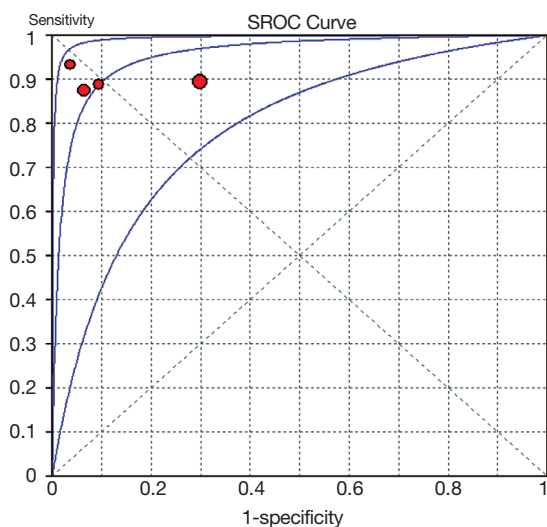
Figure 5 Summary receiver operator characteristic (SROC) of T2 relaxation time shows a symmetric curve with an AUC (area under the curve) of 0.955, Q index value of 0.897 and standard error of 0.026.
