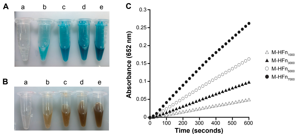
Figure 4 Peroxidase-like activity assays of M-HFn nanoparticles.
