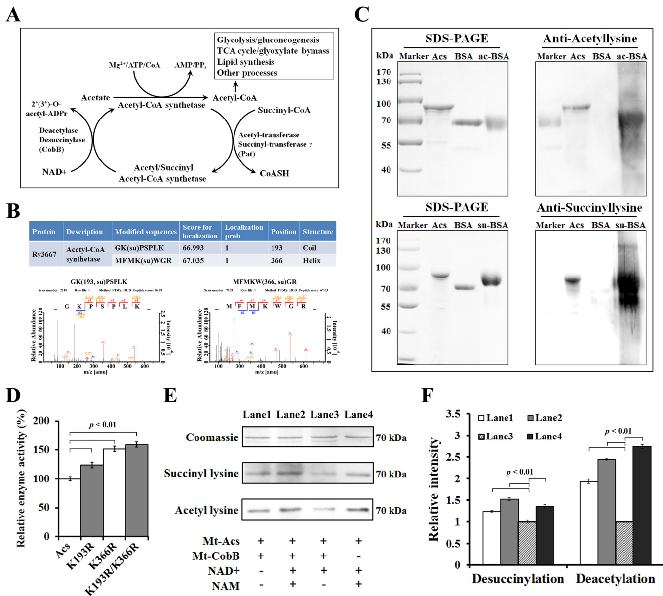
FIG. 7. Succinylation profiling of Acs of Mtb . A , Schematic illustration of regulation of Acs activity by reversible acetylation and succinylation. B , Identification of the modification sites of Acs. The representation of the corresponding MS/MS spectra of succinylated peptides from Acs annotated with a comprehensive series of b and y fragment ions. Details of succinylation sites were listed in the supplemental Table S1. C , The acetylation/succinylation levels of purified recombinant Acs were determined by immunoblotting using specific anti-acetyl/succinyl lysine antibodies. D , Succinylation of Lys193 and Lys366 affect the enzyme activity of Acs. The Acs and its mutants (Acs-K193R, Acs-K366R, and Acs-K193R/K366R) were expressed in E. coli BL21 (DE3) and the specific activity of Acs was determined. Data are means \pm S.D. from three independent assays. E , NAD + -dependent deacetylation/desuccinylation of Acs by CobB protein (Rv1151c). Acs was incubated with CobB in the presence of NAD + (0.5 mM) for 10h at 25 °C. Nicotinamide (NAM, 2 mM) was added to the reaction as CobB inhibitor. F , Quantification of acetylated/succinylated Acs in the reactions from E . Each sample was standardized by comparing to the Coomassie blue stained gel. Error bars indicate S.D. of three measurements.
