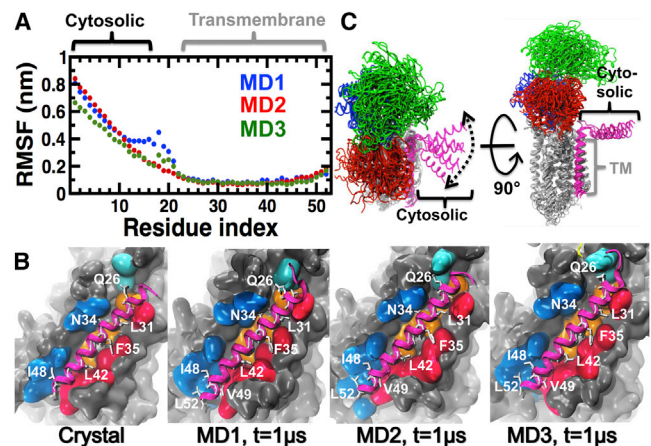
FIGURE 2 Structural characteristics of PLB in the complex. (A) \text{C}_\alpha RMSFs of PLB calculated from each independent MD trajectory. Brackets show the location of the cytosolic and TM helices of PLB. (B) Interactions between the TM domains of SERCA (surface representation) and PLB (cartoon representation) in the crystal and MD structures. PLB is colored in magenta. Residues of PLB that are important for inhibition are shown as white sticks. These residues are located at the SERCA-PLB interface. TM helices of SERCA that are directly involved PLB binding (TM2 (blue), TM4 (cyan), TM6 (orange), and TM9 (red)) are shown. (C) Cartoon representation of the structural ensembles of SERCA-PLB averaged over all three MD trajectories. SERCA and PLB are color-coded as indicated in Fig. 1. To see this figure in color, go online.
