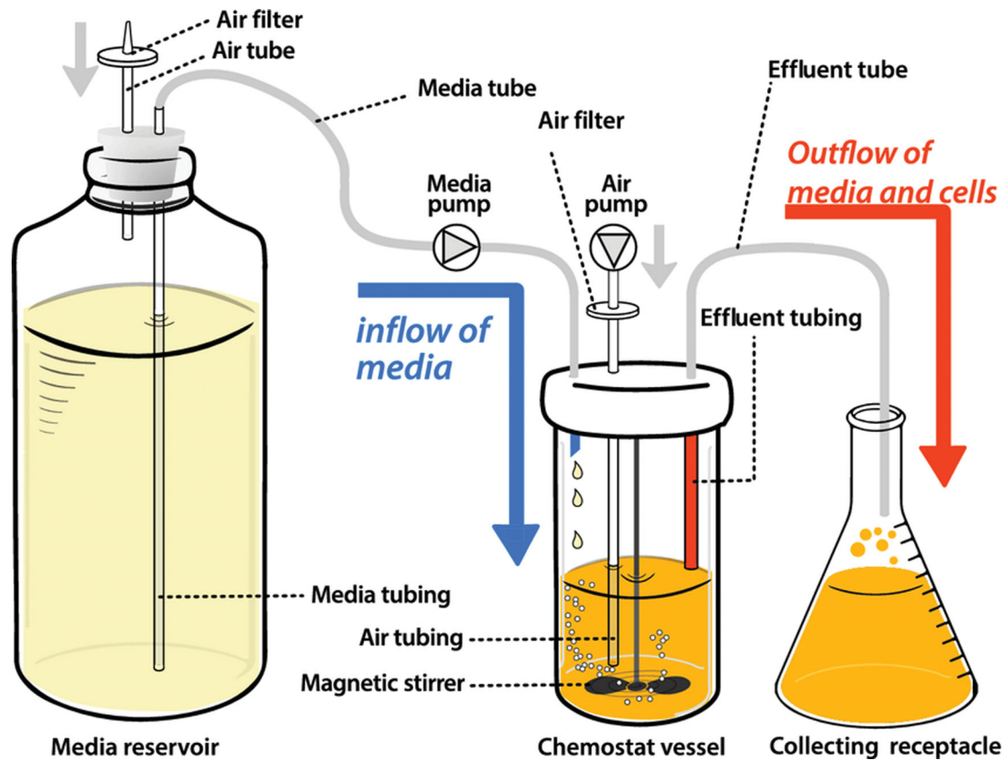
Figure 1. Design of a chemostat. Typically, a chemostat comprises a culture vessel in which the population grows under continuous agitation and aeration. New media flows into the vessel at a defined rate. At the same rate, culture containing cells and medium is removed from the chemostat. The flow of media and culture is maintained using a pumping apparatus and holding the chemostat vessel under positive pressure by means of a constant air flow.
