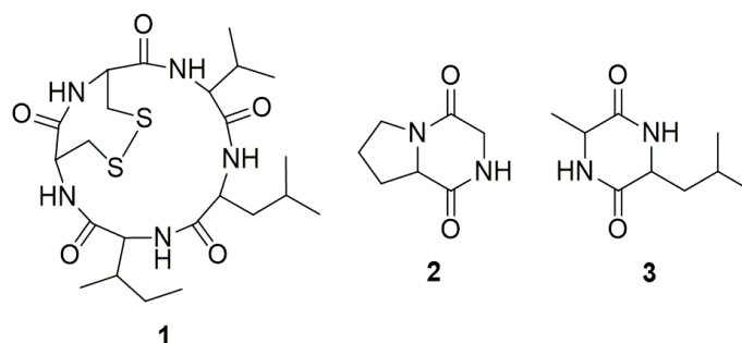
Figure 3. Chemical structures of the cyclic peptides 1–3 .
