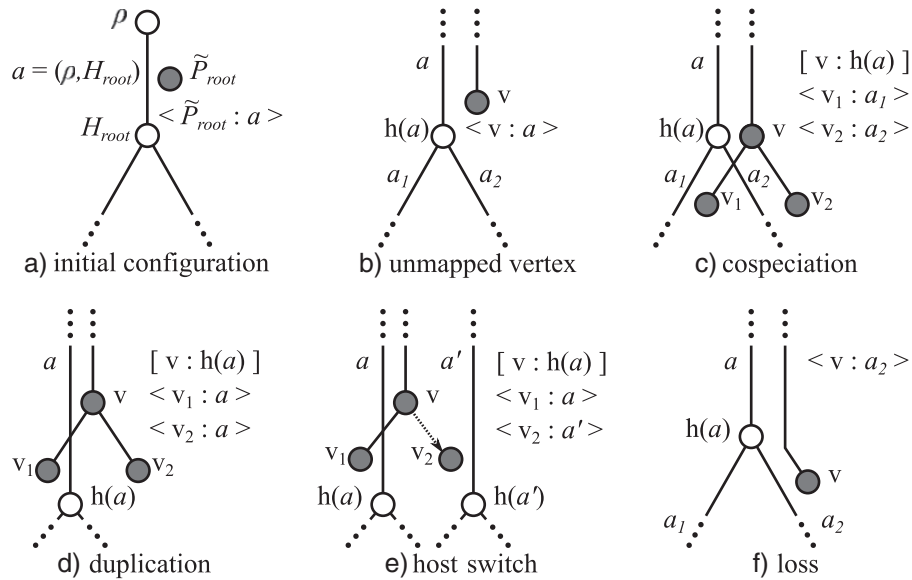
FIGURE 2. Events during the generation of the parasite tree \tilde{P} . The host tree has white vertices and the parasite tree gray vertices. The association \langle v:a \rangle indicates that an unmapped parasite vertex v is positioned on the arc a of the host tree. The association [v:w] indicates that the parasite vertex v is mapped to the host vertex w . a) initial configuration; b) unmapped vertex; c) cospeciation; d) duplication; e) host switch; f) loss.
