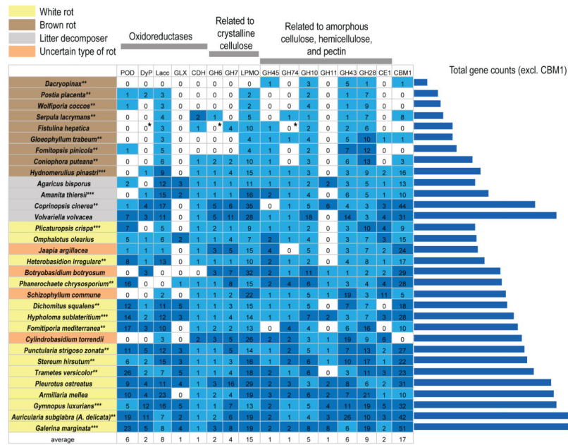
Figure 3. Copy numbers for fifteen gene families and CBM1 across 32 Agaricomycotina genomes. The columns on the right side of the table represent the summed number of genes for the fifteen gene families. Species on the table have been grouped in three categories; brown-rot (brown), litter decomposers (grey), white-rot (yellow) or uncertain type of rot (orange). Within each category, the species have been arranged based on the total number of gene copies they have. White-rot and uncertain type of rot have been grouped together for this purpose. Light blue indicates copy number below or equal to the average number of copies for the gene family, while dark blue indicates copy number above the average number of copies for the gene family. * One potential pseudogene is found for each of these gene families on the genome of F. hepatica . Data from: **Floudas et al., 2012, *** Kohler et al., unpublished data.
