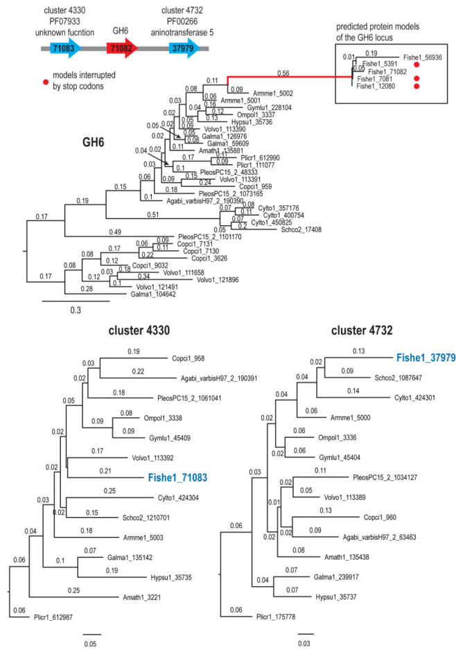
Figure 4. Phylogenetic relationships of the five predicted models of the potential GH6 pseudogene from F. hepatica with homologs from the 14 genomes showing the resulting long branch (in red color) and comparison with similar analyses of the adjacent genes. Numbers on the branches represent branch length. The scaffold graph shows the orientation of each potential pseudogene with its adjacent genes. Red dots for GH6 models of F. hepatica indicate models interrupted by stop codons. The protein models that represent the product of the adjacent genes are shown in blue on their corresponding phylogeny.
