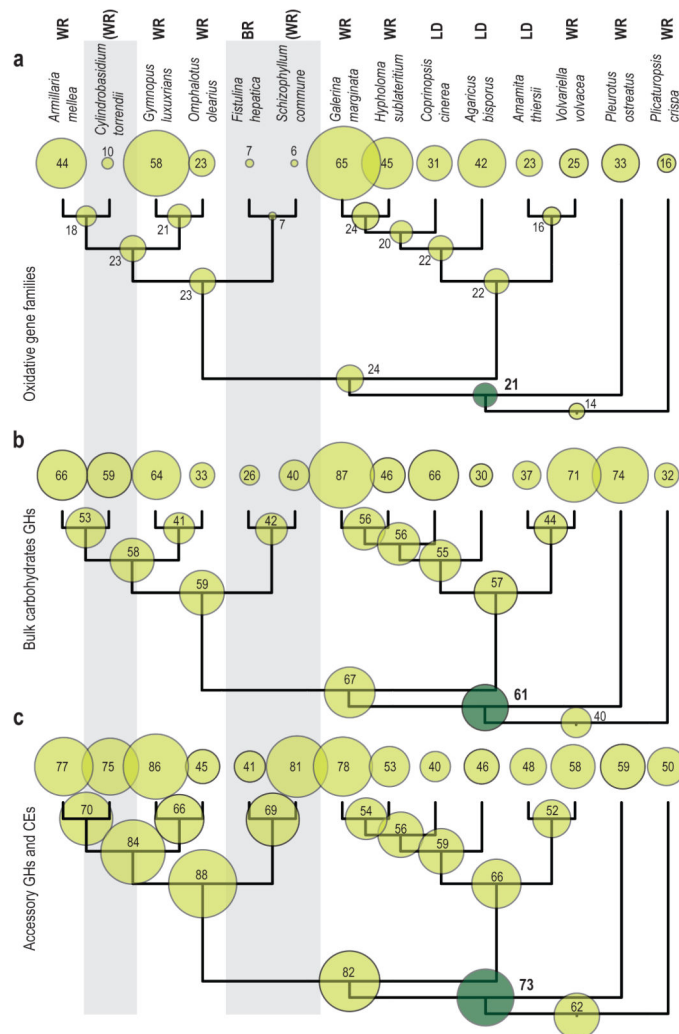
Figure 2. Species tree/gene tree reconciliation results. Summed reconciliation results of oxidative enzymes related to lignin degradation (a), bulk carbohydrate CAZY (b), and accessory CAZY (c). Numbers at the tips represent the summed number of copies for the corresponding category of gene families in the genome of each species. Numbers at internal nodes represent the predicted summed number of copies for the corresponding category of gene families for each ancestral species. The size of the circles is proportional to these numbers (shaded in dark green for the common ancestor of Agaricales). Nutritional strategies are coded as in Figure 1.
