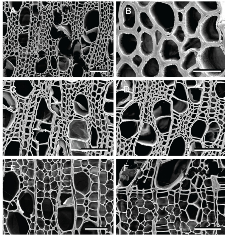
Figure 5. Scanning electron micrographs of transverse sections of aspen ( Populus ) wood decay by Cyindrobasidium torrendii (A and B), Fistulina hepatica (C and D) and Schizophyllum commune (E and F). A and B. Localized degradation of all cell wall components with erosion of the wall taking place from the cell lumen towards the middle lamella. Small voids occurred in the wood cells where all cell wall layers were degraded. C and D. A diffuse attack on wood cells resulted in cells with altered walls. No cell wall erosion took place but walls were slightly swollen and cells were partially collapsed and appeared convoluted. E and F. Thinning and eroded secondary wall layers were evident in wood cells. In some cells, the secondary wall was completely degraded but the middle lamella between cells remained. The thinned cell wall broke and detached in some areas resulting in small voids. Bar = 100 \mu\text{m} in A, 20 \mu\text{m} in B and 50 \mu\text{m} in C, D, E, F.
