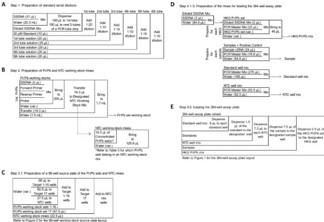
Figure 3: Schematic of specific steps in the qRT-PCR assay protocol. A-E diagram select portions of the protocol. (A) Step 1: Preparation of standard serial dilutions. (B) Step 2: Preparation of Pr/Pb and NTC working stock mixes. (C) Step 3.1: Preparation of a 96-well working stocks plate of the Pr/Pb sets and NTC mixes. (D) Step 4.1-3: Preparation of the mixes for loading the 384-well assay plate. (E) Step 4.5: Loading the 384-well assay plate. Diagrams are read from the top left to the bottom right corner. Reagents for the interferon (IFN) assay are stored at -20^{\circ}\text{C} and are listed in the left column; lines separate actions in the protocol. Please click here to view a larger version of this figure.
