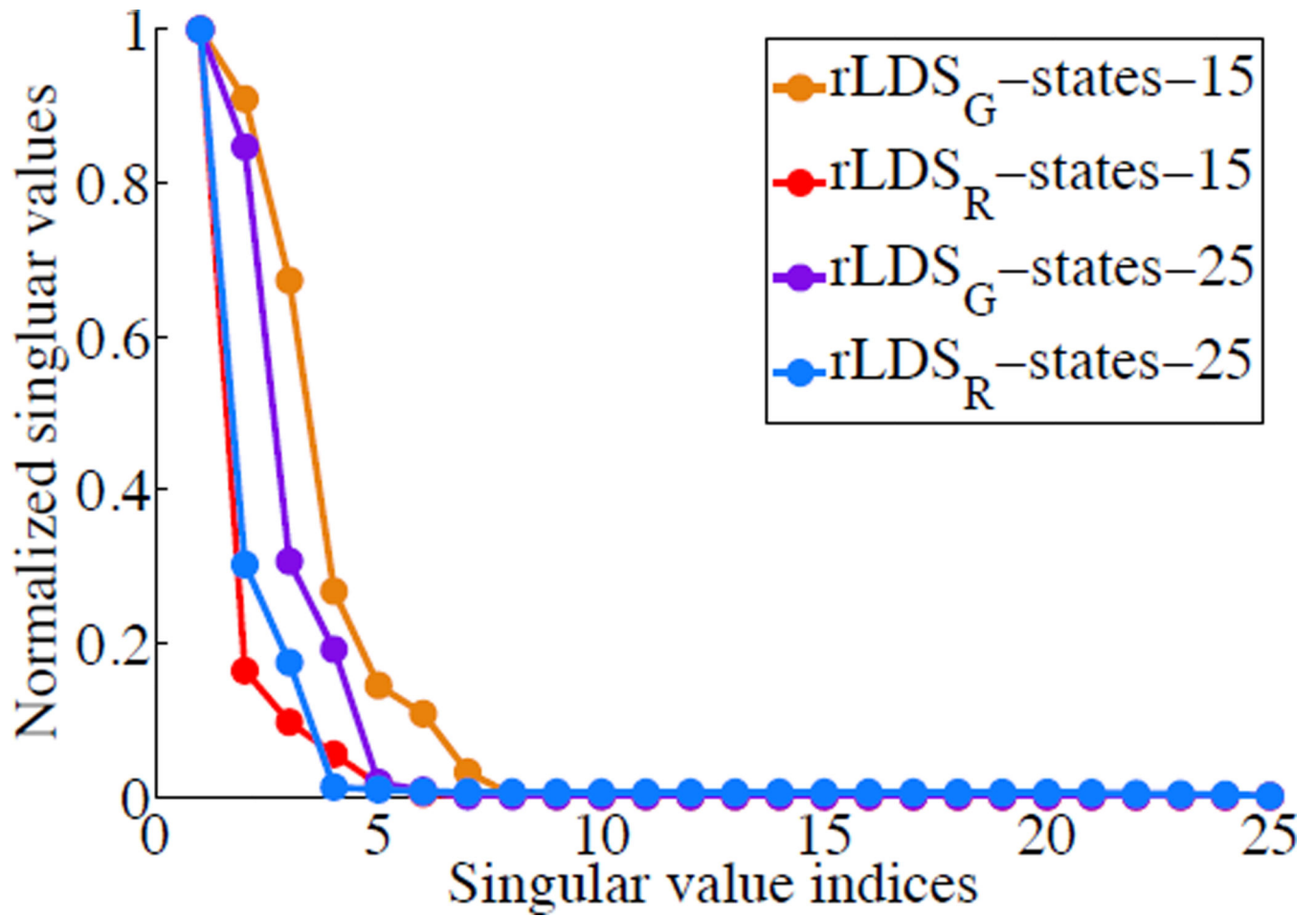
Figure 4. rLDS state size recovery.
