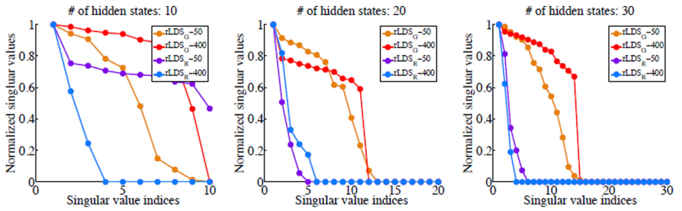
Figure 2. State space recovery on a clinical dataset.
