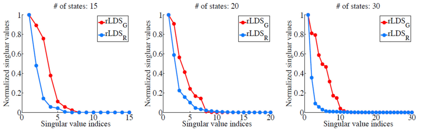
Figure 1. State space recovery on a synthetic dataset.
