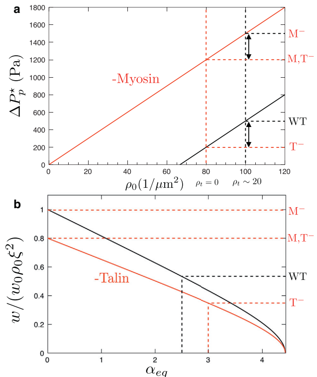
FIGURE 2 Theoretical predictions for the critical aspiration pressure and adhesion energy in a micropipette experiment. (a) Critical pressure as a function of the density of linkers \rho_0 according to Eq. 8. (Solid black and red lines) Cells with and without myosin II, respectively. (Horizontal dashed lines) Experimentally measured value of the critical detachment pressure (28) for wild-type cells (WT), mutants lacking myosin ( M^- ), mutants lacking talin ( T^- ), and double mutants ( M, T^- ). The slope and height of the two theoretical curves is entirely determined by these critical pressures (see text). (b) Effective adhesion energy as a function of the equilibrium cortical tension in the cell according to Eq. 9. (Solid black and red lines) Cells with and without talin, respectively. To see this figure in color, go online.
