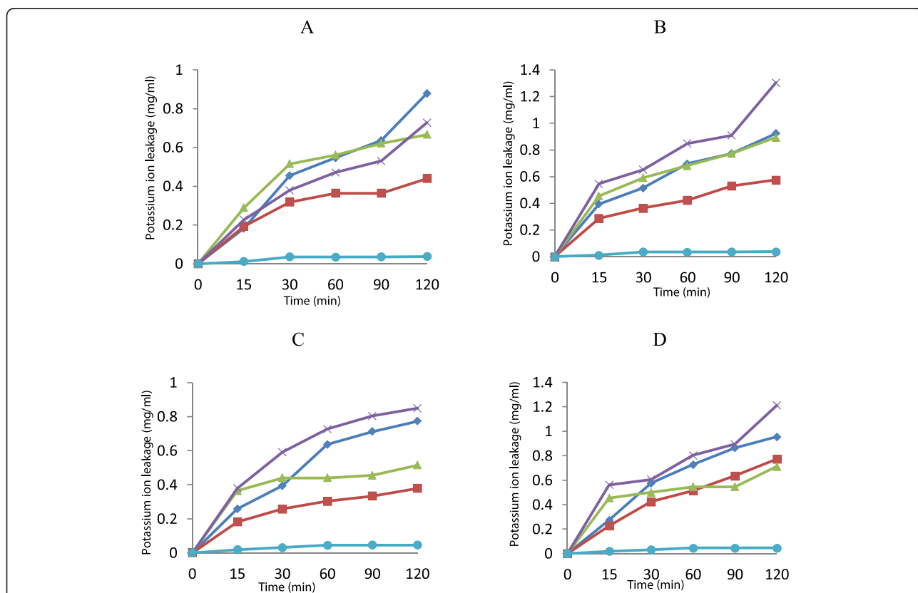
Figure 3 The effect of n-hexane fraction (◊), ethyl acetate fraction (◻), n-butanol fraction (◻), aqueous fraction (×) and control (●) on potassium ion leakage from Enterococcus faecalis (A,B) and Klebsiella pneumoniae (C,D) cells at 1 × MIC (A,C) and 2 × MIC (B, D). Each point represents the amount of potassium ions leaked (mg/ml) from cells at a particular time interval in the presence of the fractions.
