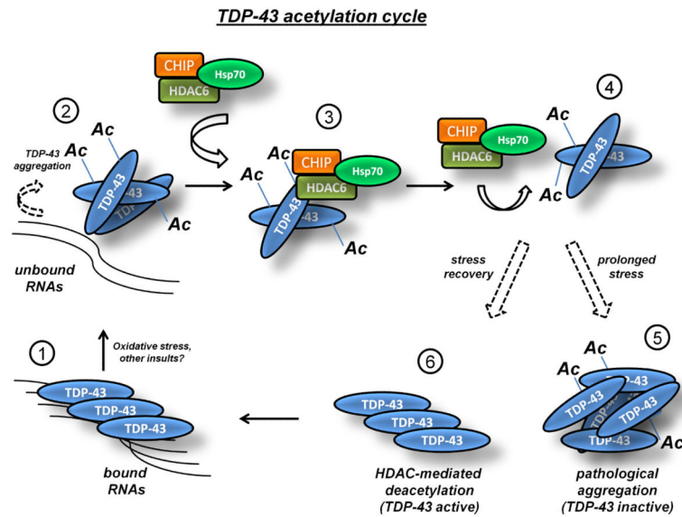
Figure 7. Model for reversible regulation of TDP-43 via lysine acetylation
