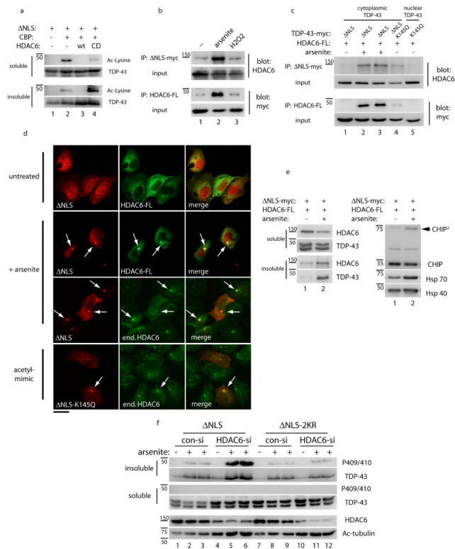
Figure 5. The deacetylase HDAC6 binds and deacetylates TDP-43 in a stress-regulated manner a) Cells were co-transfected with TDP-43- NLS, CBP, and either wild-type HDAC6 or the catalytically dead HDAC6-H611A mutant and TDP-43 acetylation was determined by immunoblotting with acetyl-lysine antibodies similar to Figure 1c. b) Cells transfected with myc-tagged TDP-43- NLS and FLAG-tagged HDAC6 were analyzed by co-immunoprecipitation reactions under basal or stimulated conditions in the presence of 0.1 mM arsenite or 1 mM peroxide stress for 2 hr. Input, representing 5% of total lysate volume, was analyzed by immunoblotting using the indicated antibodies. c) Co-immunoprecipitation analysis using either TDP-43- NLS or acetylation mimic mutants (TDP-43-K145Q or TDP-43- NLS-K145Q) and wild-type HDAC6 were performed in the absence or presence of arsenite, and immunoprecipitated proteins were analyzed by western blotting with the indicated antibodies similar to b above. d) Immunofluorescence microscopy was performed on cells expressing myc-tagged TDP-43- NLS, acetylation mimic TDP-43- NLS-K145Q, and HDAC6-FLAG where indicated, using anti-FLAG or endogenous HDAC6 antibodies. TDP-43 acetylation-mimic mutations or acute treatment with arsenite led to the formation of cytoplasmic aggregates that co-localized with HDAC6. The scale bar represents 25 \mu m. e) Protein levels of the HDAC6/CHIP/Hsp70 complex were determined by western analysis of soluble and insoluble fractions using HDAC6, CHIP, Hsp70, and Hsp40 specific antibodies. Note, CHIP dimers (arrowhead) suggest activation of CHIP E3 ligase function, as previously reported 68 . f) Depletion of HDAC6 was performed using a specific HDAC6 siRNA followed by arsenite treatment, and solubility of TDP-43- NLS and TDP-43- NLS-2KR proteins were analyzed by immunoblotting with total and phosphorylated TDP-43 antibodies. HDAC6 siRNA knock-down efficiency was validated by assessing total levels of HDAC6 and its major substrate acetylated tubulin.
