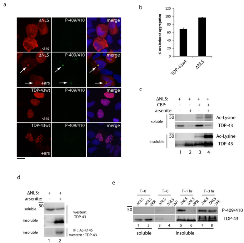
Figure 4. Oxidative stress promotes TDP-43 acetylation and pathological TDP-43 aggregation (a) Double-labeling immunofluorescence microscopy of WT TDP-43 or cytoplasmic TDP-43 was performed using anti-myc and anti-phospho-TDP-43 (P-409/410) antibodies, which illustrate TDP-43 phosphorylation and aggregation upon acute exposure to 0.2 mM arsenite for 1 hr. The scale bar represents 25 \mu m. (b) Quantification of nuclear or cytoplasmic TDP-43 stippling and aggregation phenotypes for all lysine mutants was performed from N=3 independent experiments as detailed in the methods section. Error bars represent standard error of the mean (SEM). (c) Immunoblotting of soluble and insoluble fractions using anti-myc and anti-acetyl-lysine antibodies illustrates the accumulation of acetylated TDP-43 upon co-transfection of CBP and exposure to 0.2 mM arsenite for 1 hr. (d) Immunoprecipitation reaction using Ac-K145 followed by immunoblotting with a monoclonal anti-TDP-43 antibody allowed increased sensitivity for detection of acetylated TDP-43 in the absence of CBP (see also Supplementary Figure 11). (e) Immunoblotting analysis of TDP-43- NLS and the double lysine mutant, TDP-43- NLS-2KR, was evaluated in an arsenite-induced aggregation time-course, which showed delayed accumulation of phosphorylated TDP-43- NLS-2KR aggregates compared to TDP-43- NLS.
