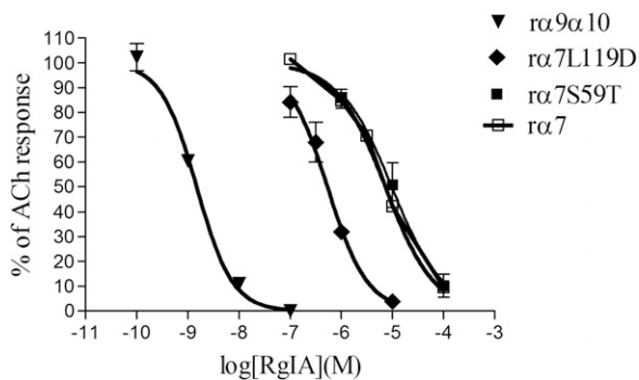
Fig. 3. Dose-response curves for \alpha -CTx RgIA on rat \alpha 9\alpha 10 , rat \alpha 7 , and rat \alpha 7 mutants \alpha 7S59T and \alpha 7L119D . There was an approximately 10-fold gain in potency of RgIA on the \alpha 7L119D receptor mutant. The concentrations of ACh used were 100 \mu M for \alpha 9\alpha 10 and 200 \mu M for \alpha 7 and \alpha 7 mutants. Data are mean ± S.E.M. from at least three separate oocytes.
