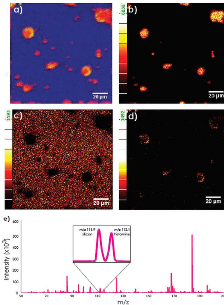
Figure 1. One compartment liposome model (histamine-containing giant liposomes) imaged with a J105 -3D Chemical Imager. Data shown are from the second layer of analysis after the first image acquisition removed the surface of the sample exposing the liposome interior. Acquisition time: 22 min/layer; pixel resolution of 500 nm/pixel, analysis area: 130 × 130 μm 2 ; 256 × 256 pixel images were acquired with a primary ion dose density of 2.42 × 10 13 ions-cm -2 /layer. a) An overlay of PC (m/z 184.1, red), silicon (m/z 111.9, blue) and histamine (m/z 112.1, green). b) Ion image of PC at m/z 184.1. c) Ion image of silicon at m/z 111.9. d) Ion image of histamine at m/z 112.1. e) Mass spectrum from image showing the two peaks at m/z 112.
