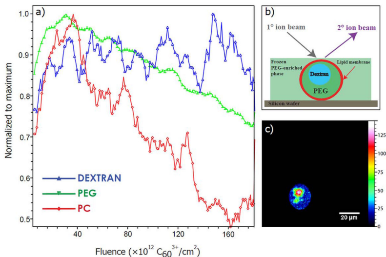
Figure 3. Depth profile of two-compartment liposome model across the ATPS containing giant liposome. a) ToF-SIMS sputter depth profile acquired with the TOF.SIMS V. Acquisition time: 97.16 s; fluence: 3.33 \times 10^{13} \text{ Bi}_3^+ / \text{cm}^2 ; FoV ( \text{Bi}_3^+ ): 105 \times 105 \mu\text{m}^2 ; FoV ( \text{C}_{60}^{3+} ): 200 \times 200 \mu\text{m}^2 . b) Schematic of liposome embedded in frozen PEG-enriched phase. c) Depth profile was reconstructed from the specific region of interest.
