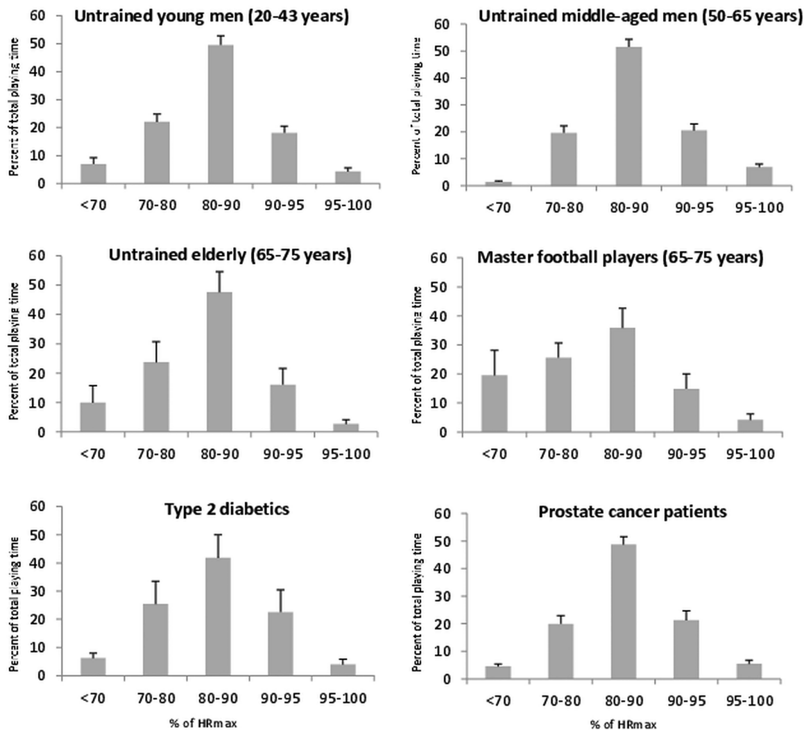
Figure 1 Heart rate distribution, expressed as a percentage of maximum heart rate, during football training consisting of small-sided games for various study groups. Data are presented as means±SEM. HRmax, maximal heart rate.
