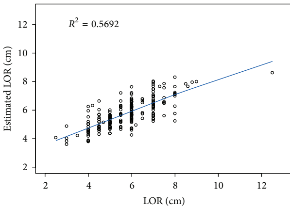
FIGURE 4: Correlation between measurements (cm) of loss of resistance (LOR) and skin to epidural space depth determined from computed tomography (SES-CT), adjusted for demographic and anthropometric factors.
