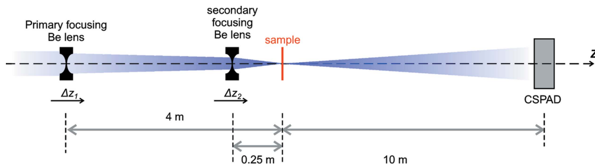
Figure 1 Schematic of the focusing setup used at the XPP instrument. The X-ray beam is focused by either a single set of beryllium compact refractive lenses nominally located 4 m upstream of the sample (labeled as ‘primary focusing’) or by two sets of lenses installed 4 m and 0.25 m upstream of the sample (‘primary’ and ‘secondary’ focusing). Both lenses are installed on motorized stages to allow translation along the beam propagation direction by \Delta z_1 and \Delta z_2 , respectively.
