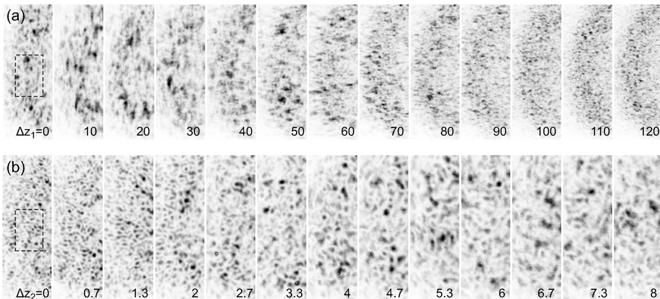
Figure 2 (a) Speckle patterns measured at different lens positions \Delta z_1 for the single CRL set configuration. (b) Speckle patterns measured at different lens positions \Delta z_2 for the double CRL set configuration, with the position of the primary lens remained fixed at z_1 = 4 m. The shown portions of the scattering patterns are centered around q = 0.05 \text{ nm}^{-1} . All patterns are 120 shot (1 s) averages. Lens positions are indicated at the lower right-hand corners of each pattern in millimeters. The dashed rectangle in both \Delta z = 0 images indicates the region of interest used for subsequent speckle size analysis.
