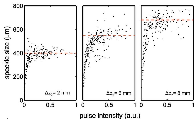
Figure 4 Calculated speckle size in the vertical direction versus pulse intensity for the double CRL focusing case at three different secondary lens positions \Delta z_2 . From left to right: 2 mm, 6 mm and 8 mm.
