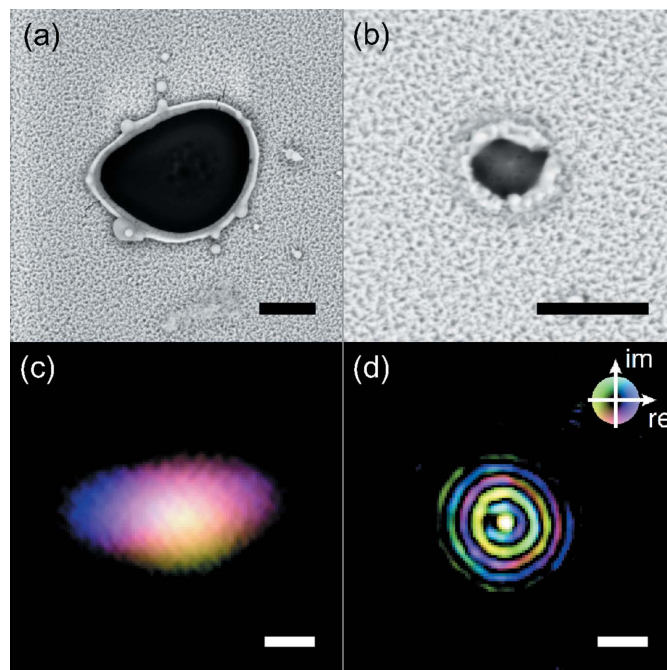
Figure 6 Beam focus measurement examples from imprints and ptychographic reconstructions. All scale bars are 1 \mu\text{m} in size. (a) Single CRL set focusing imprint. (b) Double CRL set focusing imprint. (c) Ptychographic reconstruction for single CRL set focusing. (d) Ptychographic reconstruction for double CRL set focusing. The color scale for both ptychographical reconstructions (c) and (d) are shown in the upper right-hand corner of (d), with the brightness and the color representing the amplitude and the phase, respectively.
