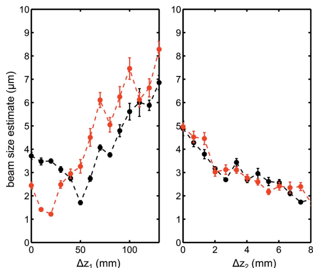
Figure 5 Derived beam sizes at sample location from speckle sizes, horizontal d_x (black circles) and vertical d_y (red circles). Left: beam sizes versus \Delta z_1 for the single CRL set focusing. Right: beam sizes versus \Delta z_2 for the double CRL set focusing.
