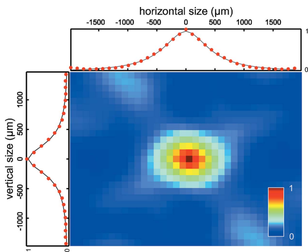
Figure 3 Calculated spatial autocorrelation function from a single-shot speckle pattern for the double CRL set focusing case at \Delta z_2 = 8 mm. Horizontal and vertical lineouts through the center of the autocorrelation and their Lorentzian fits are plotted around the image.
