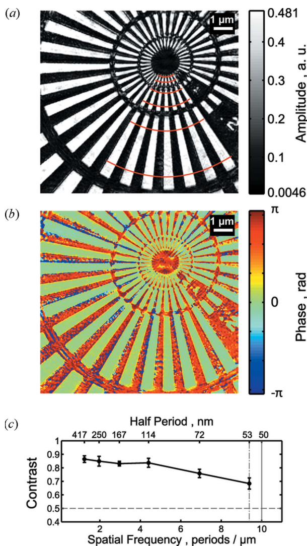
Figure 6 Ptychographic reconstruction of the Siemens star test pattern. (a) Amplitude and (b) phase image. (c) Contrast C between high and low transmission as a function of spatial frequency from the angular scans denoted by red lines in the amplitude image.
