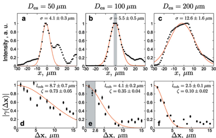
Figure 3 Results of coherence measurement in the vertical direction for three exit slit openings D_{es} at 500 eV. Black dots indicate measured data and dashed lines represent Gaussian fits. (a)–(c) Intensity profiles measured with scans of a 1.5 \mu\text{m} pinhole. (d)–(f) Modulus of the CCF |\gamma(\Delta x)| . The gray shaded areas in (b) and (e) indicate the coherent part of the beam selected by the beam-defining 2.6 \mu\text{m} pinhole. The r.m.s. values \sigma of the beam size obtained from Gaussian fits, the coherence length l_{coh} , as well as the values of the global degree of coherence \zeta determined from equation (4) are also shown. For the Gaussian fits we used the data points up to 9 \mu\text{m} in (e) and up to 7 \mu\text{m} in (f).
