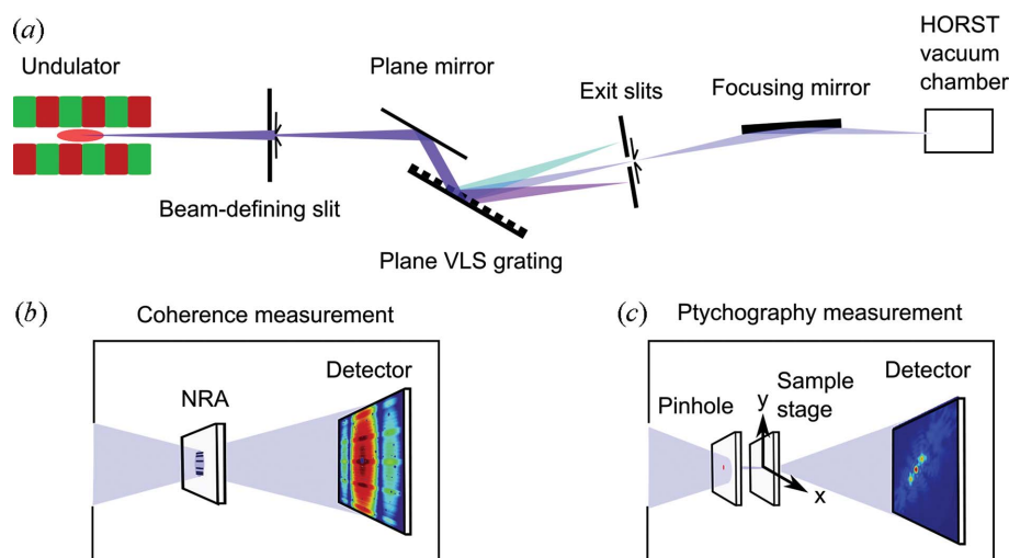
Figure 1 (a) Soft X-ray beamline layout. The X-ray scattering vacuum chamber HORST in the coherence measurement setup (b) and the ptychography setup (c).
