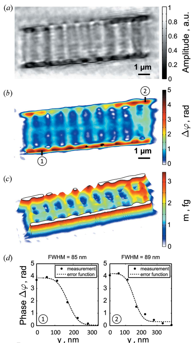
Figure 7 Ptychographic reconstruction of the amplitude (a) and the phase (b) of the fossil diatom. (c) Integrated SiO 2 mass along the depth of the diatom (see text for further details) and (d) FWHM values of two error function fits along the black lines indicated in the phase reconstruction in (b).
