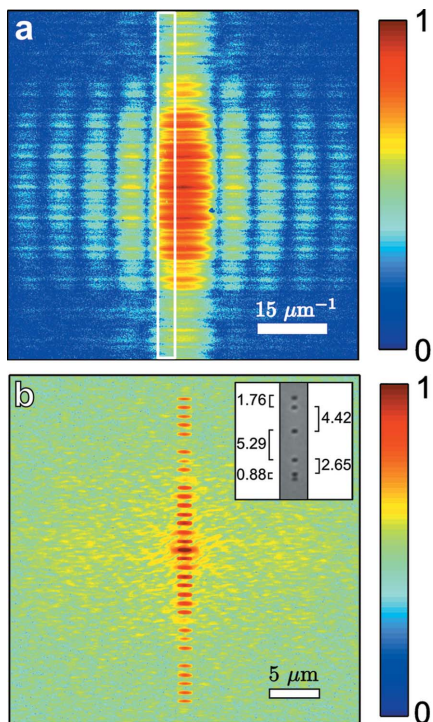
Figure 2 (a) Diffraction pattern from a vertically oriented NRA measured at 500 eV and D_{es} = 100 \mu\text{m} . The white rectangle indicates the area used for the analysis. (b) The Fourier transform of the NRA diffraction pattern. Both images are displayed on a logarithmic scale. (Inset) Optical microscope image of the NRA and its aperture separations shown in micrometers.
