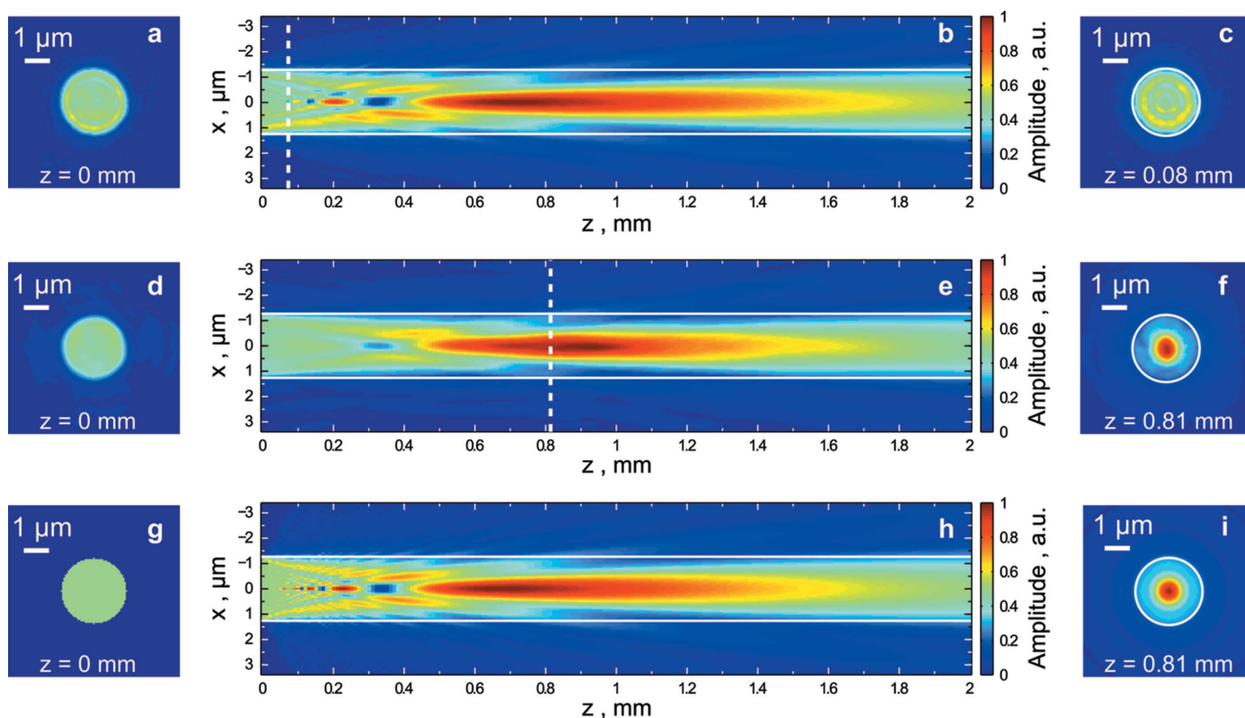
Figure 5 Ptychographic probe function reconstruction from the Siemens star ( a–c ) and the diatom ( d–f ). A plane wave simulation for propagation of the wavefield from a 2.6\ \mu\text{m} pinhole aperture is shown in ( g, h, i ). Amplitude distribution at the position of the pinhole ( a, d, g ); distribution of the wavefield amplitude downstream of the pinhole ( b, e, h ); amplitude distribution of the probe amplitude at the position of the sample ( c, f, i ) [Siemens star ( c ), and diatom ( f )]. The simulated amplitude distribution ( i ) is shown at the same z position as for ( f ). Dashed white lines in ( b, e ) indicate the position of the sample relative to the pinhole at z = 0 . White circles in ( c, f, i ) indicate the pinhole size.
