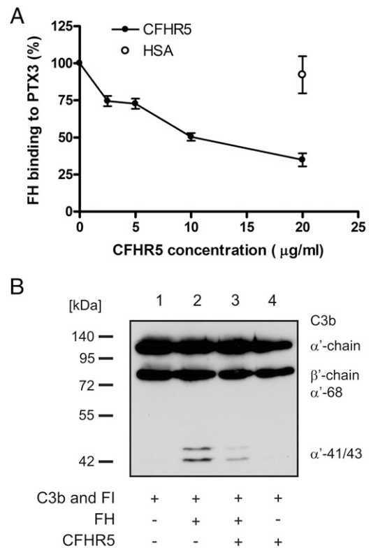
FIGURE 5. CFHR5 competes with FH binding and activity on PTX3. (A) The binding of 50 \mu g/ml ( \sim 300 nM) FH to PTX3 was measured in the presence of increasing concentrations of CFHR5 (up to 20 \mu g/ml, corresponding to \sim 300 nM CFHR5) using an FH-specific mAb for detection. HSA was used as control protein. The normalized values are means \pm SD derived from four independent experiments. The binding of FH was significantly different in the presence of 20 \mu g/ml CFHR5 than in the presence of 20 \mu g/ml HSA ( p = 0.0005, unpaired t test). (B) The cofactor activity of FH bound to PTX3 for the cleavage of C3b in the presence and absence of CFHR5 was measured by Western blot as described in Materials and Methods . Microplate wells were coated with 10 \mu g/ml PTX3 and incubated with 50 \mu g/ml FH with or without 20 \mu g/ml CFHR5, as indicated below the blot, and then C3b and FI were added to each well. The molecular mass marker is indicated on the left, and the C3b chains and the C3b \alpha' -chain cleavage fragments are indicated on the right. The blot was developed using HRP-conjugated C3-specific Ab that recognizes C3b and its fragments but not C3d. The blot is representative of three independent experiments.
