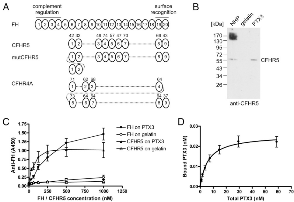
FIGURE 1. CFHR5 interacts with PTX3. (A) Schematic drawing of FH, CFHR5, and CFHR4A. FH is built up of 20 CCP domains, of which CCPs 1–4 mediate complement regulatory activity and CCPs 19–20 mediate surface recognition by FH. The CCP domains of CFHR5, and also CFHR4A, which was used as control protein in several experiments, are shown aligned with the corresponding most related FH domains. The numbers above the domains indicate the percentage of amino acid sequence identity between the homologous domains. The mutant CFHR5 protein detected in CFHR5 nephropathy and containing a duplication of CCPs 1–2 is also shown. CFHR4B consists of CCPs 1 and 6–9 of CFHR4A (not shown). (B) Microplate wells were coated with gelatin or PTX3 and then incubated with 25% normal human plasma (NHP). After washing, bound proteins were removed by adding SDS sample buffer and subjected to 10% SDS-PAGE and Western blotting using monoclonal anti-CFHR5. The blot is representative of three experiments. (C) Comparison of binding of CFHR5 and FH to PTX3. Immobilized PTX3 and gelatin, used as negative control protein, were incubated with the indicated concentrations of purified FH or recombinant CFHR5. Binding of both proteins was detected by an FH Ab. Data are means ± SEM derived from four experiments. Both FH and CFHR5 bound to PTX3 significantly stronger than to gelatin ( p < 0.001, two-way ANOVA). (D) Addition of increasing amounts of PTX3 results in a saturable binding to immobilized CFHR5. Specific binding was measured using a standard curve of PTX3. Data are means ± SEM from eight experiments.
