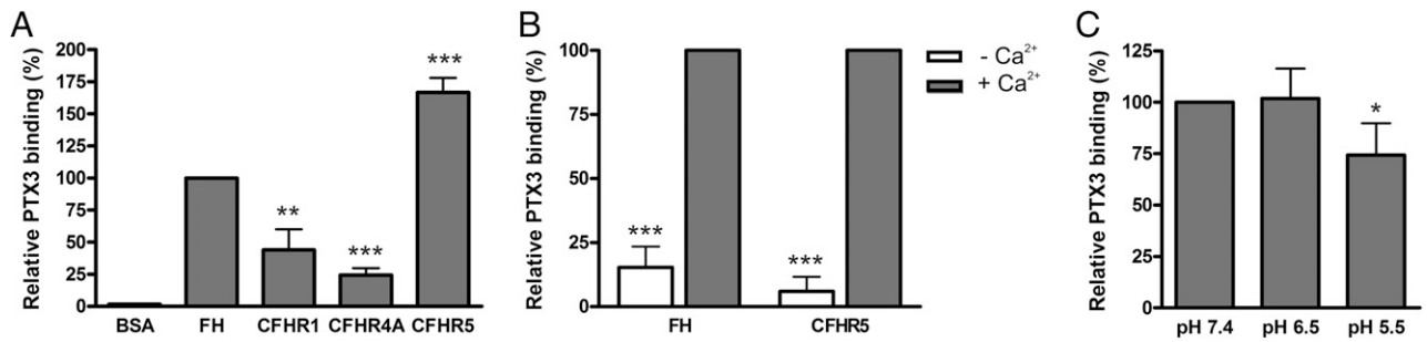
FIGURE 2. Comparison of the binding of PTX3 with CFHR proteins, and dependence of the PTX3–CFHR5 interaction on calcium concentration and pH. (A) Binding of PTX3 to recombinant CFHR5 was compared with that of CFHR1, CFHR4A, and FH by ELISA. The FH family proteins and BSA, used as negative control, were immobilized in equimolar concentrations (200 nM) in microplate wells, and then 5 \mu\text{g}/\text{ml} recombinant PTX3 was added for 1 h at 37°C. PTX3 binding was determined using a polyclonal anti-PTX3 Ab. The values were normalized for FH binding (100%) and show means \pm SD derived from three independent experiments. ** p < 0.01 , *** p < 0.001 , one-way ANOVA. (B) The binding of PTX3 to immobilized FH and CFHR5 was compared in DPBS (pH 7.4) with (filled bars) and without (open bars) 1 mM \text{Ca}^{2+} . The data are normalized to binding in the presence of \text{Ca}^{2+} (100%) and represent means \pm SD from four experiments. *** p < 0.001 , one-way ANOVA. (C) The binding of PTX3 to CFHR5 was compared in TBS with pH 7.4, 6.5, and 5.5. The data shown are normalized to values obtained with TBS pH 7.4 (100%) and represent means \pm SD from five experiments. * p < 0.05 , one-way ANOVA.
