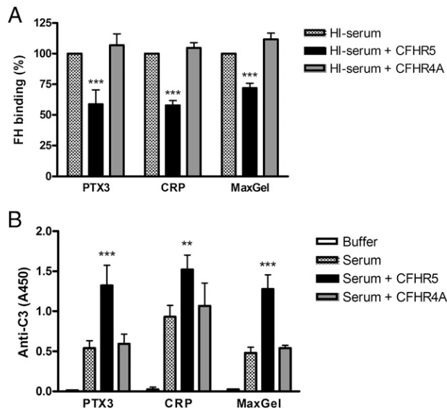
FIGURE 8. CFHR5 competes with FH in serum for binding to PTX3, CRP, and MaxGel and causes enhanced C3 fragment deposition. (A) Wells were coated with 10 \mu\text{g/ml} PTX3, 10 \mu\text{g/ml} CRP, and MaxGel diluted 1:30 in DPBS. After blocking, the wells were incubated for 30 min at 37°C with 25% heat-inactivated human serum with or without 0.5 \mu\text{M} CFHR5 and CFHR4A. FH binding was detected with mAb A254 and the corresponding secondary Ab. The normalized values are means \pm SD derived from three independent experiments. *** p < 0.001, one-way ANOVA. (B) Nunc microplate wells were coated with 10 \mu\text{g/ml} PTX3, 10 \mu\text{g/ml} CRP, and MaxGel diluted 1:30 in DPBS. After blocking, 12.5% normal human serum (for PTX3 and CRP) and 25% normal human serum (for ECM) were added for 30 min at 37°C, with or without 20 \mu\text{g/ml} CFHR5 or CFHR4A. Complement activation was detected by measuring C3 fragment deposition using HRP-conjugated goat anti-human C3. Data represent mean absorbance values \pm SD from three independent experiments. ** p < 0.01, *** p < 0.001, one-way ANOVA.
