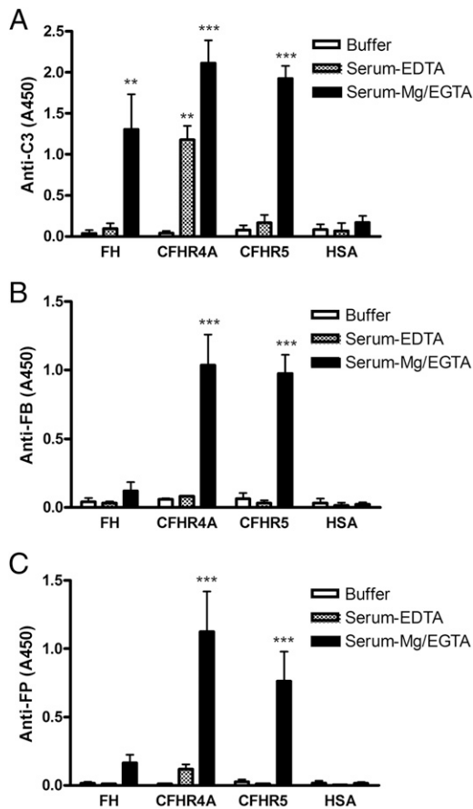
FIGURE 10. Complement activation by CFHR5. CFHR5 was immobilized on microplate wells and incubated with 10% normal human serum in 5 mM Mg 2+ -EGTA buffer to allow only alternative pathway activation or with 10% serum containing 5 mM EDTA to inhibit complement activation. Deposition of (A) C3b, (B) FB, and (C) properdin (FP) was detected using the corresponding Abs. Immobilized CFHR4A was used as positive control and FH and HSA were used as negative controls. The data are means \pm SD derived from three independent experiments. ** p < 0.01 , *** p < 0.001 , one-way ANOVA.
