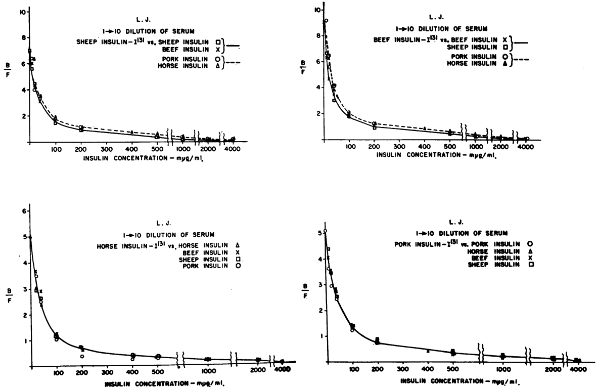
FIG. 3. SUBJECT L. J. RATIO OF BOUND INSULIN- I^{131} TO FREE INSULIN- I^{131} ( B/F ) AS A FUNCTION OF CONCENTRATION OF VARIOUS UNLABELED INSULINS
