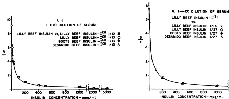
FIG. 6. B/F RATIOS FOR VARIOUS I 131 -LABELED INSULINS AS A FUNCTION OF THE CONCENTRATION OF UNLABELED LILLY BEEF INSULIN IN L. J. (LEFT) AND B/F RATIOS FOR LILLY BEEF INSULIN - I 131 AS A FUNCTION OF CONCENTRATION OF DIFFERENT PREPARATIONS OF UNLABELED BEEF INSULIN IN G. (RIGHT)
