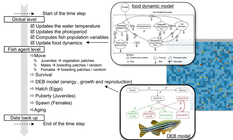
Fig 1. Schema of the schedule of the model of zebrafish population dynamics. Schema of food sub-model was issued from Li and Yakupitiyage [61] and schema of the dynamic energy budget (DEB) model was issued from Kooijman [21]. An arrow before an action denotes that action was realized in random order by fish agents one after another in swift succession.
