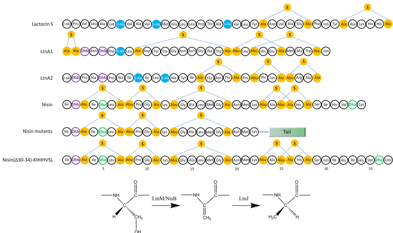
FIG 1 Structures of lactocin S, lactacin 3147 (peptides LtnA1 and LtnA2), nisin, nisin with designed C-terminal tail, and nisin(Δ30-34)-KIHIVSL. The residues involved in the formation of (methyl)lanthionine are in yellow, D-alanines are depicted in blue, and Dha and Dhb are colored green and purple, respectively. The pathway for D-alanine conversion from serine is depicted. 2-ob, 2-oxobutyryl group.
