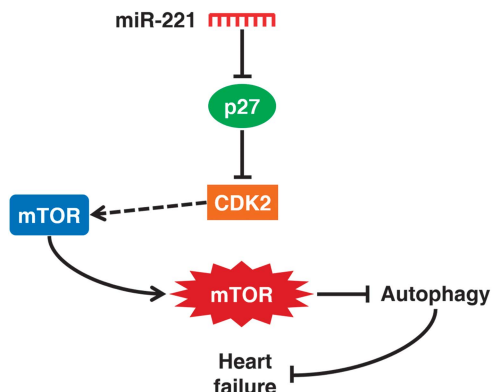
Figure 8 MiR-221 induces heart failure by inhibiting autophagy. Model depicting the downregulation of p27 expression by miR-221, resulting in CDK2-dependent mTOR activation, which inhibits autophagy to provoke heart failure
