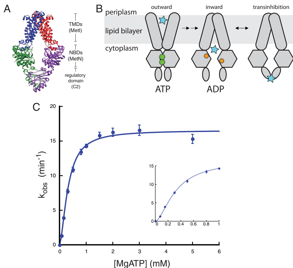
FIGURE 1. Binding of ATP to MetNI is cooperative. A , representation of MetNI structure and domains within the cell membrane (11). B , alternating access model for transport with the addition of the transinhibition model. C , ATPase activity of MetNI in the absence of inhibitors. Inset , observed rate constant at low concentrations of MgATP. Reaction conditions consisted of 60 mM Tris, pH 7.5, 5 mM TAPS, pH 8.5, 0.05% DDM, 55 mM NaCl, 200 \mu\text{M} 2-amino-6-mercapto-7-methylpurine riboside, 0.1 units of purine nucleoside phosphorylase per 100 \mu\text{l} , and equimolar amounts of \text{MgCl}_2 and ATP at 33 ^\circ\text{C} . Equations for fitting are described under "Experimental Procedures." Error bars represent S.E. from at least three independent experiments.
