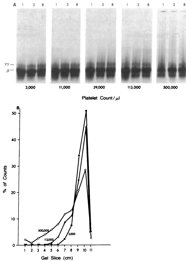
Figure 4. (A) SDS-2% agarose electrophoresis of fibrin clots prepared with increasing platelet counts and for different incubation intervals. PRP and plasma with a platelet count of 3,000/ \mu l were prepared from five normal donors and mixtures made to adjust the platelet counts as shown. After addition of radiolabeled fibrinogen, clots were prepared for 1, 3, and 8 h; dissolved; and aliquots subjected to electrophoresis. A total of 60,000 counts was applied to each lane, and autoradiography was for 20 h. (B) Distribution of radioactivity in polypeptide chains of fibrin prepared for 8-h plasma clots at varying platelet counts after SDS-2% agarose gel electrophoresis. 8-h plasma clots prepared from plasma with platelet counts of 3,000/ \mu l, 113,000/ \mu l, and 500,000/ \mu l were electrophoresed as shown in A. After staining, drying, and autoradiography, the gel was sliced at intervals and the proportion of radioactivity in each slice calculated. The \gamma\gamma -chains were located in slices 8 and 9, the \alpha -monomer in slices 9 and 10, and \beta -chain also in slices 9 and 10.
