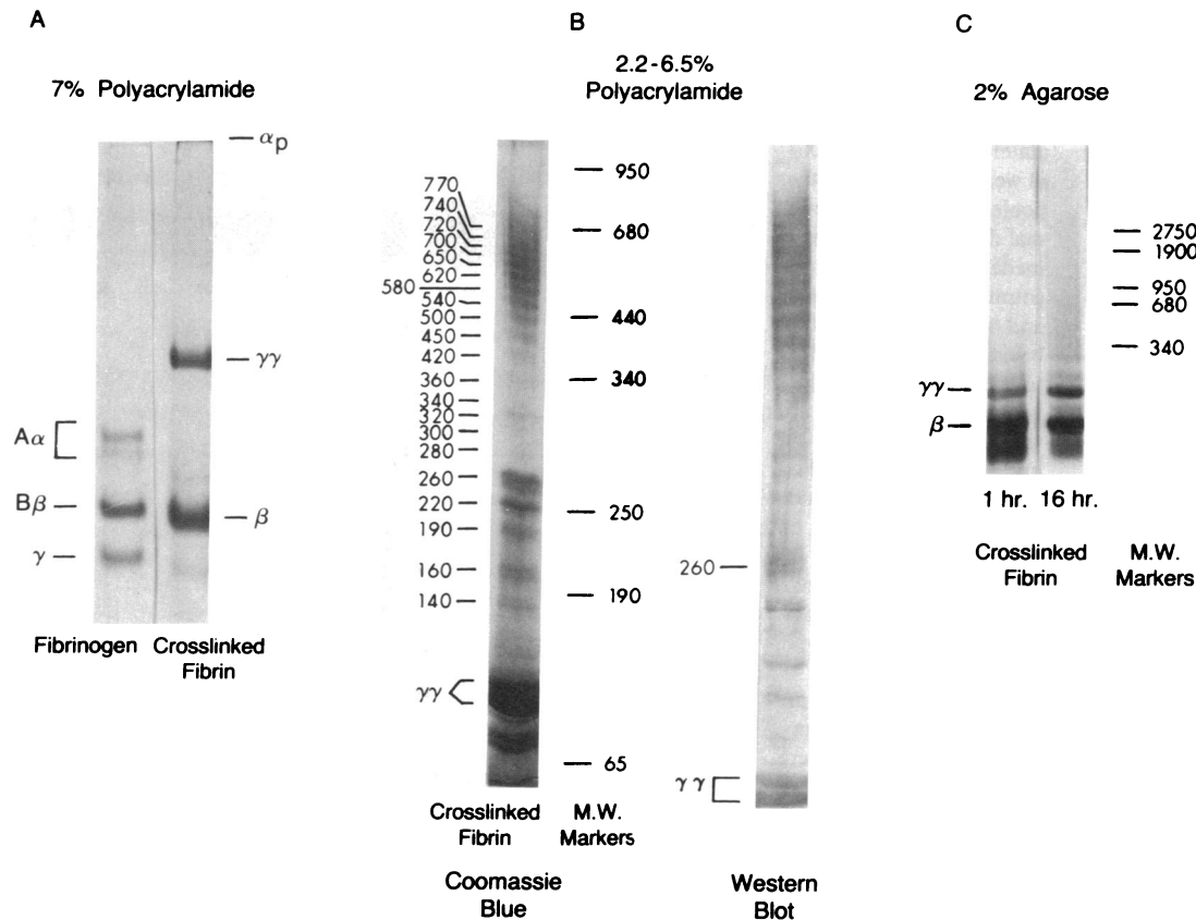
Figure 1. Electrophoresis of reduced cross-linked fibrin in different gel systems. (A) SDS-7% polyacrylamide gel of purified fibrinogen and a 1-h fibrin clot prepared from pooled normal plasma (10 \mu g each). \alpha -polymer chains are represented by nonentering protein at the top of the gel and by several faint bands migrating more slowly than the \gamma\gamma -chain. (B) Electrophoresis in an SDS-2.2-6.5% polyacrylamide gel of fibrin (60 \mu g) prepared by clotting pooled normal plasma for 1 h. The 2% stacking gel was lost in preparation. Electrophoresis proceeded until the \gamma\gamma -chains were near the bottom of the gel and the \beta -chain had exited. The locations of unreduced molecular weight standards electrophoresed on the same gel are indicated
