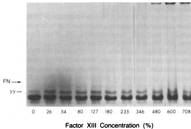
Figure 5. SDS-2% agarose electrophoresis of 3-h plasma clots prepared with increasing Factor XIII concentrations. Pooled plasma from five normal donors was centrifuged to prepare plasma containing no identifiable platelets, and the Factor XIII activity in this standard sample was taken to be 100%. Plasma containing 0% Factor XIII was obtained from a patient with a severe congenital deficiency of Factor XIII. Plasmas with Factor XIII concentrations of 26, 54, and 80% were obtained by mixing the platelet-free normal plasma and the Factor XIII-deficient plasma. Plasma containing Factor XIII concentrations above 100% was prepared by adding a Factor XIII concentrate to the standard plasma. The Factor XIII concentrations shown were determined by direct assay of plasma. Approximately 60,000 counts were added to each lane and the autoradiogram was exposed for 24 h. FN indicates the migration position of the fibronectin subunit ( M_r of 220,000) located on the protein-stained gel but not seen on the autoradiogram.
