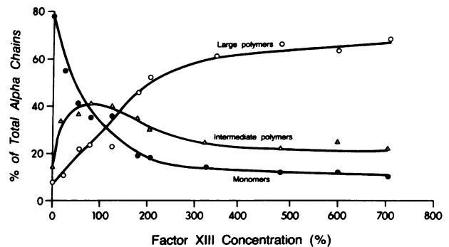
Figure 6. Proportion of monomeric and polymeric \alpha -chain forms in fibrin prepared at increasing Factor XIII concentrations. Fibrin was prepared from plasma with varying concentrations of Factor XIII and electrophoresed in SDS-7% polyacrylamide gels. After staining, drying, and autoradiography the proportion of counts migrating in different positions was determined. The \alpha -monomer was taken to represent counts between the \gamma\gamma - and \beta -chains. The largest \alpha -polymer forms were those contained in the 1st 1 cm, and intermediate sized \alpha -polymer forms were those migrating from 1 cm to the \gamma\gamma -chain position. Factor XIII concentrations were determined by assay. Factor XIII concentrations between 0 and 100% were adjusted by mixing Factor XIII-deficient plasma with pooled normal plasma containing no platelets, whereas Factor XIII concentrations above 100% were achieved by adding purified placental Factor XIII. Proportions of \alpha -monomer, intermediate polymers, and large polymers are expressed in comparison to the total \alpha -chain content in each sample.
