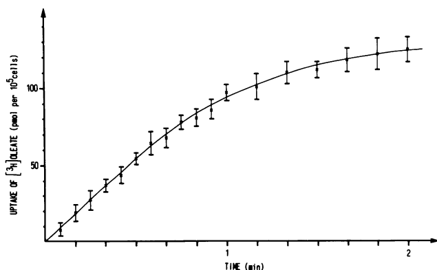
Figure 1. Time course of [ 3 H]oleate uptake. 173 μM [ 3 H]oleate/albumin (1:1) in 1 ml PBS were incubated at 37°C with 125 μl of isolated cardiomyocytes (2 × 10 6 cells/ml). At the times indicated uptake was terminated as described. Values are means±SD of three replicate experiments.
