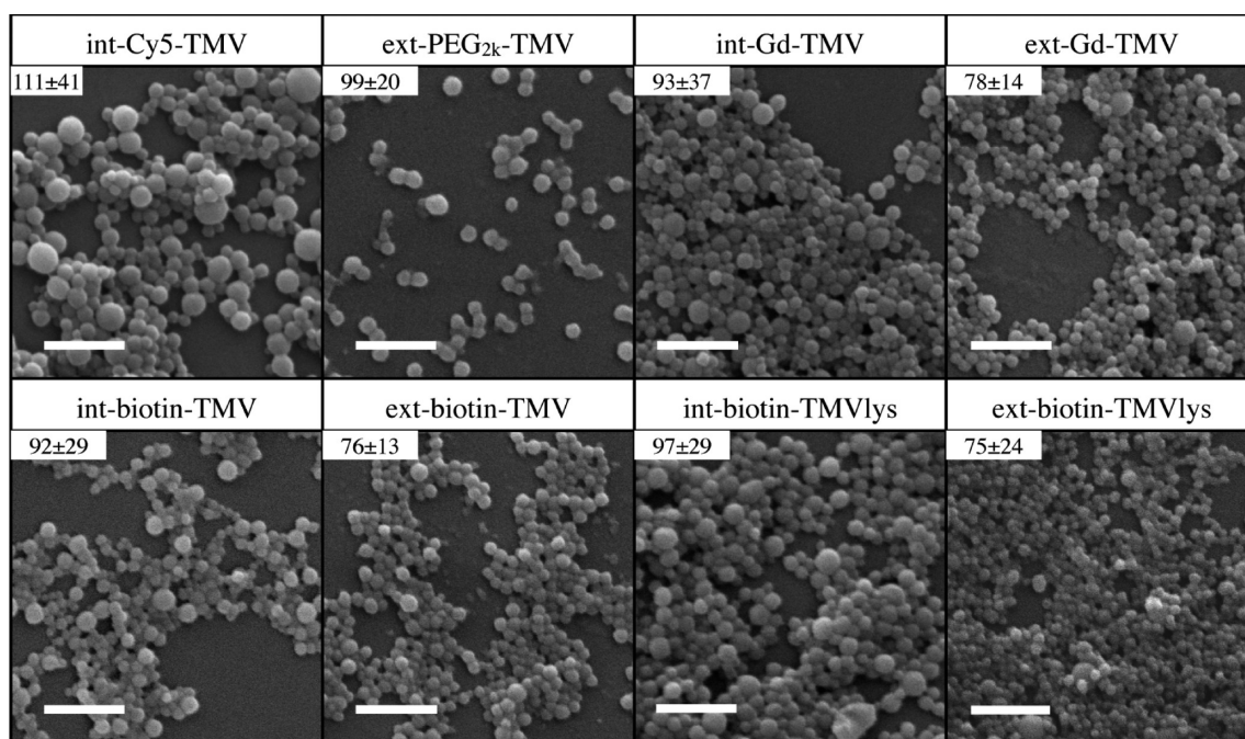
Figure 3. SEM images of SNPs formed from chemically modified TMV particles. Inset shows average diameter and standard deviation. Scale bars are 500 nm.
