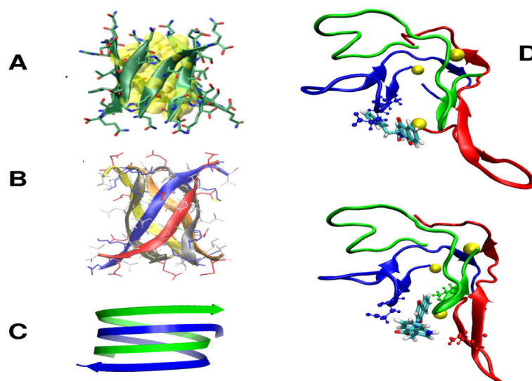
Fig.3. Amyloids. (A) The \beta -barrel of the \beta 2m(82-87) peptide as predicted by OPEP. 79,143 (B) The hexamer of the KV11 peptide consisting of six antiparallel \beta strands forming a barrel as determined by X-ray crystallography. 144 (C) The predicted OPEP antiparallel double stranded poly-L-glutamine nanotube. 145 (D) Two binding modes of the NQTrp drug to the A \beta 17-42 trimer as predicted by our multiscale simulation. The yellow balls indicate the 17th amino acids and the drug is shown with all-atoms. 96 Top view also shows all atoms of A21 and E22; bottom view shows all atoms of E22 (blue) and V39 (green).
