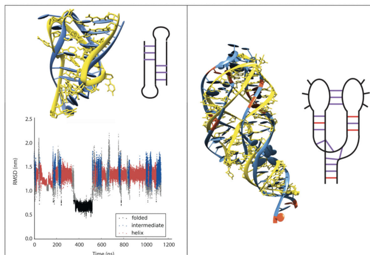
Fig.10. Hire-RNAv3 results. Left, Folding of the 22-nt pseudo-knot (2G1W) using ST simulation with the predicted state (blue) superposed on the NMR structure (yellow). The RMSD with respect to the NMR structure over time is shown. Right, MD-predicted structure of the 79-nt guanine riboswitch 1Y26 (blue) superposed on the experimental structure (yellow) using our four restraints (in red). In both panels the secondary structure of the system is shown on the right.
