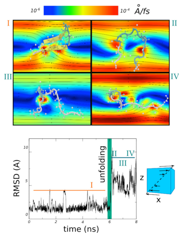
Fig.9. Time evolution of the RMSD and snapshots of a \beta -hairpin peptide (PDB code 1PGB, fragment 41-56) simulated in laminar shear flow. The velocity gradient is generated along the Z direction and corresponds in our simulation to a shear rate of \dot{\gamma} = 10^{10} \text{ s}^{-1} . We show the detailed structures of the peptide prior to unfolding (I) and at various unfolding stages (II-IV), with the velocity field represented in background and a colour scale given in the top of the figure.
