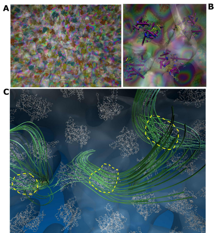
Fig.6. MUPHY/OPEP suspension. (A) Snapshot highlighting the Rat1 proteins and the solvent velocity field shown in transparency. (B) A zoom showing the Rat1 secondary structures and the local solvent velocity field. (C) Flow streamlines generated by three selected proteins in the suspension in a single timeframe.
