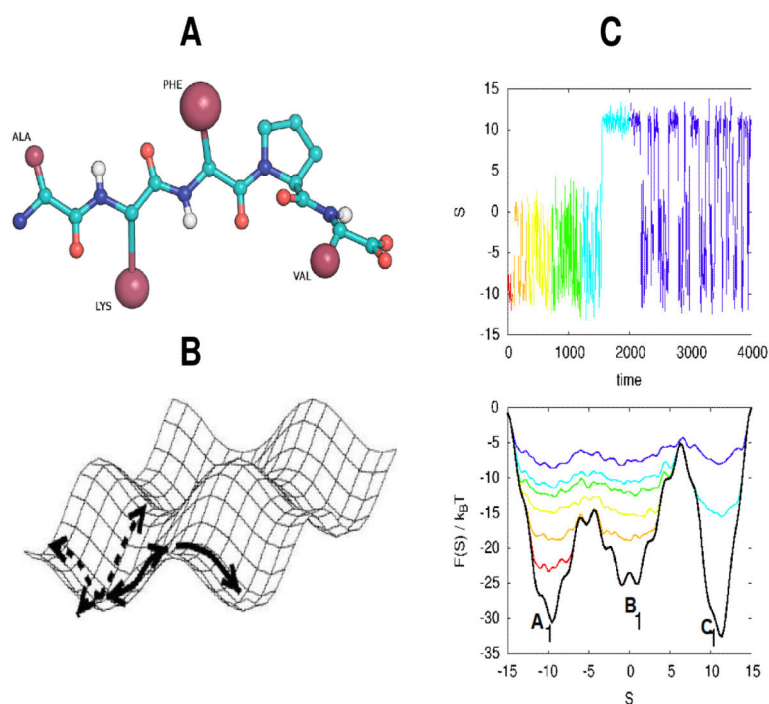
Fig.1. OPEP CG model and enhanced sampling methods. (A) We use the peptide Ala-Lys-Phe-Pro-Val in its zwitterion form to show the details of the backbone and the side-chains. (B) The Activation-Relaxation Technique connecting local minima by first-order saddle points. (C) Example of a metadynamics simulation in a one-dimensional landscape with multiple metastable minima separated by energy barriers. Top panel: System trajectory in CV space as a function of simulation time. Bottom panel: Progressive filling (colored lines) of the underlying potential (black line) by bias. In both the panels color code is used to measure the simulation time. The system starts in the basin A1 and it is pushed by the bias to overcome the free-energy barriers and to visit basin B1 ( t \sim 100 ) and basin C1 ( t \sim 1500 ). In the second half of the simulation, the system can easily sample the whole landscape and the bias can be used to estimate the underlying free-energy surface.
