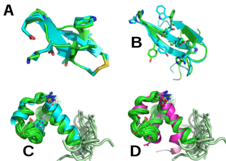
Fig.4. Structure predictions superposed on the experimental structures. (A): Best Pep-fold model of the peptide code PDB 1n0a (11-aa, BC score = 0.94) with one S-S bond; (B): Best Pep-fold model of the peptide 1e0m (37-aa, BC score = 0.88). In (A) and (B), we show the all-atom representation of some side chains; (C) and (D): Best Pep-fold and Rosetta models of the peptide 2j8p (49-aa, BC scores = 0.93 and 0.88) superposed on the 20 NMR structures and showing the flexibility of one extremity. Green: experimental conformations.
