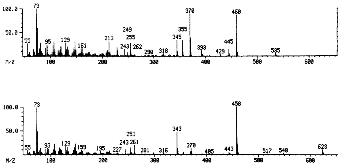
Figure 5. The electron impact (70 eV) ionization mass spectrum of the Me-TMS ether derivatives of two 5\alpha -bile acids present in the serum of twins with familial giant-cell hepatitis and identified as allo -chenodeoxycholic acid (upper) and allo -cholic acid (lower) contaminated with traces of chenodeoxycholic because of incomplete chromatographic resolution of these two bile acids).
