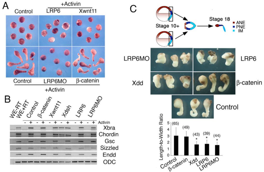
Fig. 2. Loss and gain of Lrp6 function in explants affects convergent-extension movements (A) lrp6 mRNA (LRP6; 1 ng) or Lrp6 MO (LRP6MO; 40 ng) injections block activin-mediated animal cap elongation, in a similar manner to injection of Wnt11 (400 pg) control. By contrast, injection of β-catenin at levels that cause complete axis duplication (50 pg) has no effect. (B) RT-PCR analysis shows that mesendodermal markers ( Xbra , Chordin , Goosecoid , Sizzled , Endodermin ) are induced by activin in animal caps and their expression is unaffected by injections of Lrp6 MO or lrp6 mRNA. Note induction of Xbra and Chordin after injections of similar amounts of dsh mRNA (1 ng). Loading control: ODC (ornithine decarboxylase). (C) Keller sandwiches elongate when DMZ explants are cultured in apposition. Keller sandwiches injected with Lrp6 MO (40 ng) or lrp6 mRNA (1 ng) show impaired elongation (compared to control uninjected or β-catenin expressing explants) and resemble those expressing Xdd (2 ng). ANE, anterior neural ectoderm; PNE, posterior neural ectoderm; IM, involuting mesoderm. Student's t -test was used for statistical analysis. Error bars indicate standard deviation. Asterisks mark differences that are statistically significant from control ( P < 0.01 ). Numbers of explants scored are indicated in parentheses.
