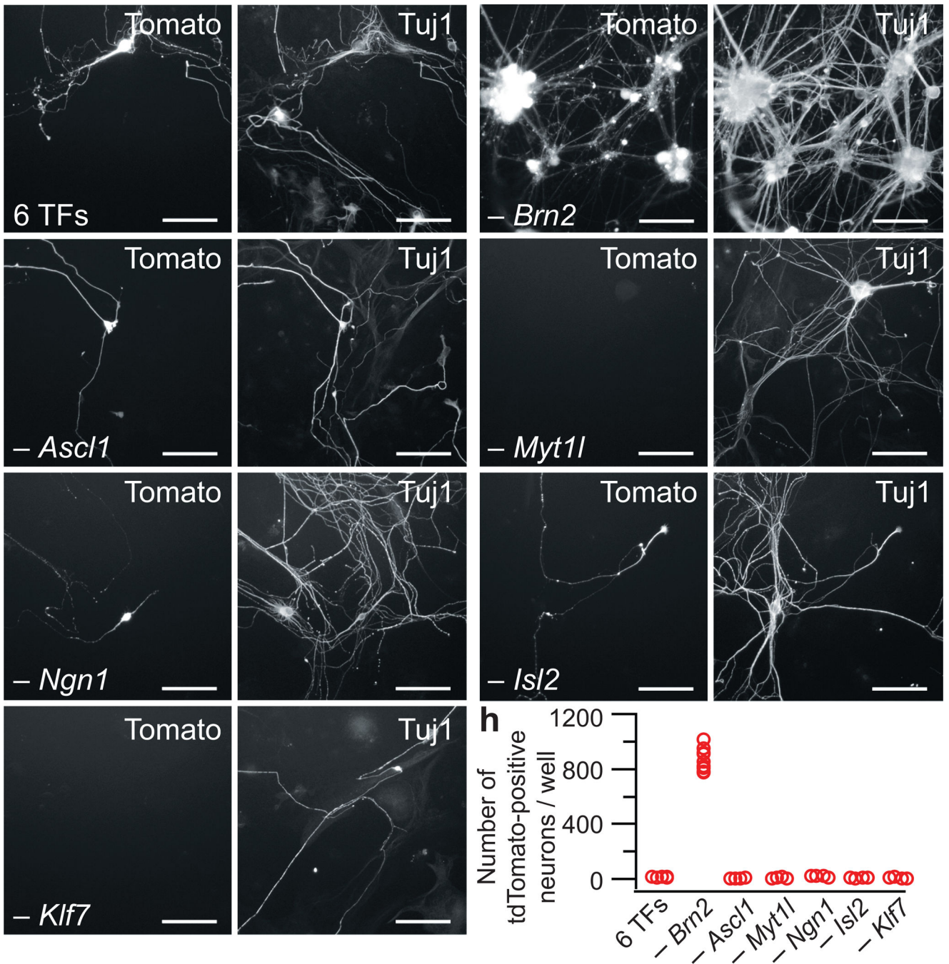
Figure 1. Combinations of transcription factors result in nociceptor production. (a) Few tdTomato, Tuj1-positive neurons are produced by the combination of six factors (6 TFs): Brn2 , Ascl1 , Myt1l , Ngn1 , Isl2 and Klf7 . (b) Removal of Brn2 markedly increases the number of tdTomato, Tuj1-positive neurons. (c–g) Omission of Ascl1 (c), Myt1l (d), Ngn1 (e), Isl2 (f) or Klf7 (g) from the six factors disrupts the generation of nociceptor neurons. Representative images for each transcription factor drop out were taken from n=4 wells from two separate
