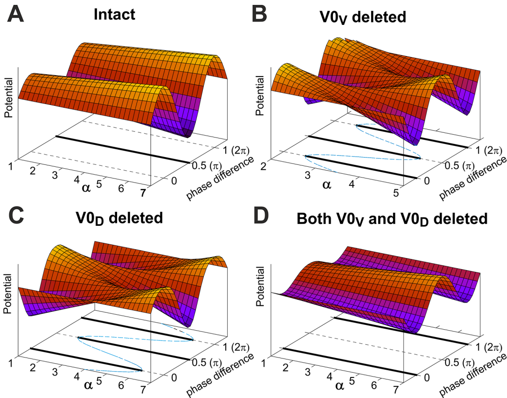
Fig 9. Interpretation of system behavior in terms of phase synchronization. A potential function for Eq (24), P(\phi) (see text for the definition), is depicted as a function of phase difference and the excitation parameter, \alpha , together with the bifurcation diagram (at the bottom) for each case: A. Intact model; B. V_{0V} connections are deleted; C. V_{0D} connections are deleted; D. Both V_{0V} and V_{0D} are deleted. Note that the phase difference is normalized to 1, i.e. \Delta\phi = \phi / 2\pi and \Delta\phi = 0.5 of the phase difference corresponds to alternation ( \phi = \pi ), whereas \Delta\phi = 0 or 1 corresponds to synchronization ( \phi = 0 or 2\pi ). Bifurcation diagrams show the coordinates of the fixed points depending on \alpha on the (\alpha, \phi) -plane. Stable equilibria are shown by thick solid lines, and unstable states are on the dashed lines. Same states can be recognized as valleys and hills on the potential surface at particular values of \alpha . For example, in the case of V_{0D} deleted, at \alpha = 1 we start with out-of-phase (alternating) regime (phase dif. \Delta\phi = 0.5 ) being a hill. As \alpha increases, the surface bends into a shallow valley around this point, which progressively gets deeper. In contrast, valleys that correspond to in-phase synchronization (phase dif. \Delta\phi = 0, 1 ) become more and more shallow, and eventually turn to hills, which signifies stability loss. Parameters used to calculate the potential surfaces and bifurcation diagrams: V_3^0 = 4 ; V_3^1 = 2 ; V_{0V}^0 = 0 ; V_{0V}^1 = 3 ; V_{0D}^0 = 11 ; V_{0D}^1 = 0 . See text for more details.
