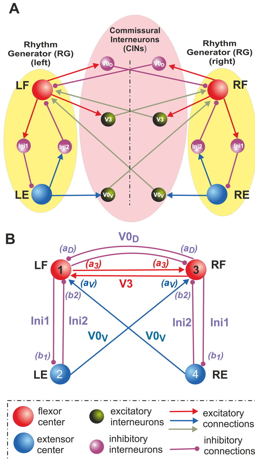
Fig 1. Organization of locomotor CPGs and commissural interactions. A. Hypothetical schematic of flexor-extensor and commissural left-right interactions between the locomotor centers. Rhythm generator (RG) in each side of the cord consists of one flexor (left, LF, and right, RF) and one extensor (left, LE, and right, RE) center that reciprocally inhibit each other via inhibitory populations of neurons (Ini1 and Ini2 on each side). Left and right RGs interact via populations of commissural interneurons (CINs). In the proposed model, three types of CINs are considered: excitatory V3 that mediate excitatory connections between LF
