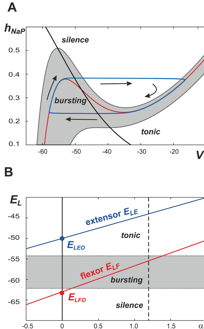
Fig 2. Operating regimes of single center and generation of rhythmic bursting. A. Representation of single center dynamics (blue line) in the (V, h_{NaP}) plane. The V -nullclines with varying E_L values are represented by the gray band and the red line; the h_{NaP} -nullcline is shown by a black line. Bursting occurs when the value of E_L is such that the V -nullcline exists within the gray region. Silence and tonic behaviors occur at values of E_L that place the V -nullcline above and below the gray region, respectively. B. It is suggested that neuronal excitability is defined by the leak reversal potential, E_L , which linearly increases with the parameter \alpha representing NMDA concentration. Bursting occurs when E_L is greater than -62.7 mV and less than -54.2 mV (gray area). Silence and tonic behaviors are observed at values below and above this range, respectively. It is suggested that the basal value of E_L (at \alpha = 0 ) for the flexor centers ( E_{LFO} ) is below the bursting area, so that with an increase of \alpha the flexor centers can generate bursting once the flexor E_{LF} is in the gray area. In contrast, the basal value of E_L for the extensor centers ( E_{LEO} ) is much higher and these centers, if disconnected, operate in a mode of tonic activity. A dashed line at \alpha = 1.2 denotes the maximal \alpha value used in our simulations.
