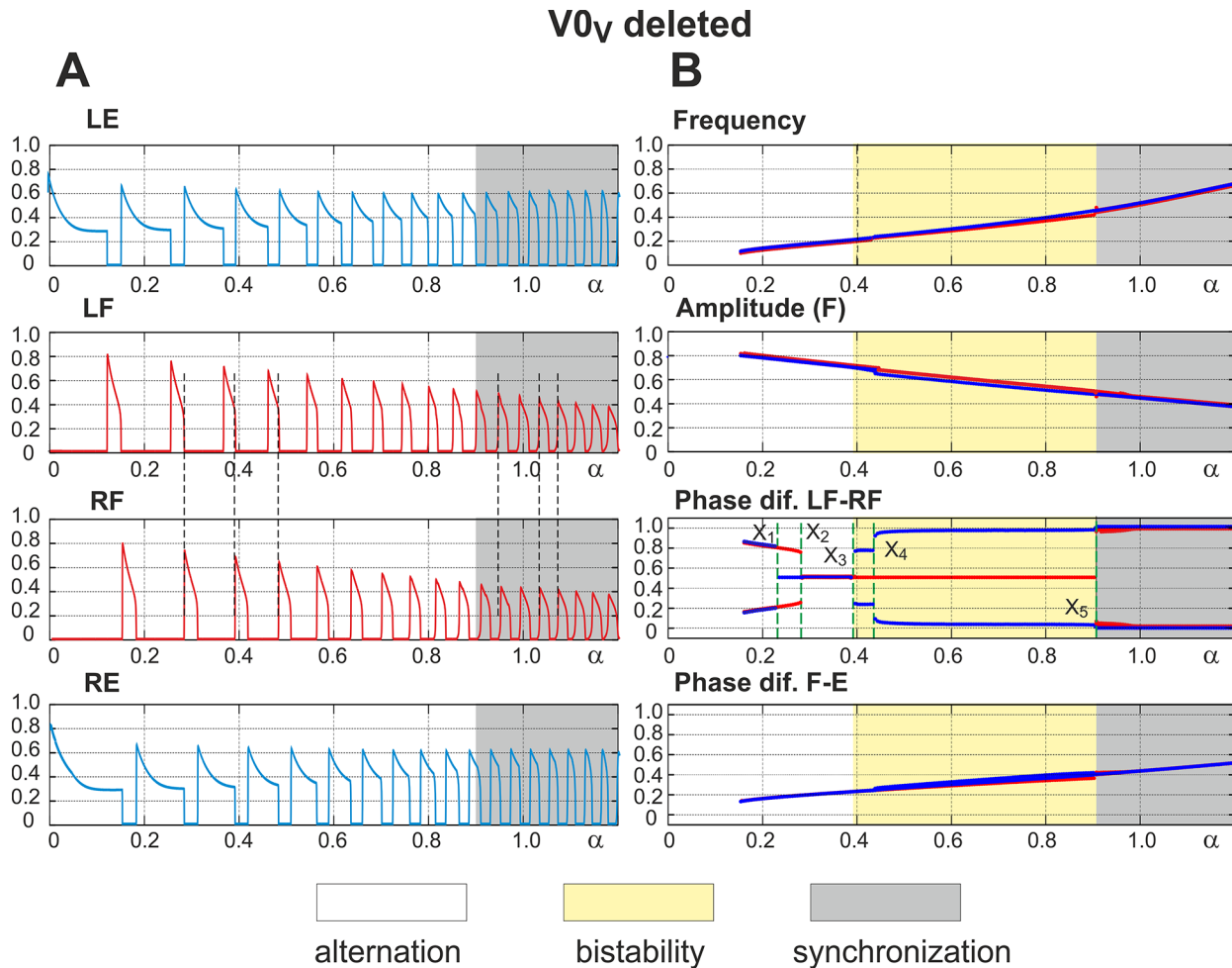
Fig 5. Performance of the model with the excitatory V0_v pathways removed. A. Changes in the activity of the four centers with increasing neuronal excitation ( \alpha ). Vertical dashed lines indicate left-right alternation of flexor center activity at low values of \alpha and its synchronization at \alpha > 0.9 . B. Bifurcation diagrams. Frequency and amplitude of flexor center oscillations change similar to the intact case (see Fig 3 for comparison). \alpha was changed in both directions, first forward from 0 to 1.2 (red lines) and then backward from 1.2 to 0 (blue lines). The non-overlapping branches indicate bistability. A series of such bistable regions exist in the diagram showing phase differences between the flexor centers ( Phase dif. LF-RF ). They are described in the text. In general, at low values of \alpha ( \alpha < X_3 \approx 0.39 ), we have different forms of left-right alternation (see text for details), at \alpha < X_5 = 0.9 there is a perfect left-right synchronization, and in the middle ( X_3 < \alpha < X_5 ) the system exhibits a bistable behavior.
