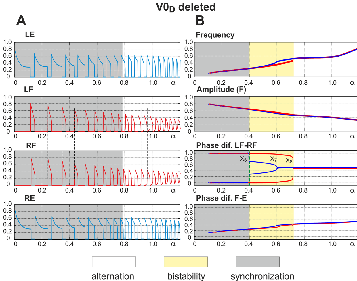
Fig 7. Performance of the model with the inhibitory V0 D pathways removed. A. Changes in the activity of the four centers with increasing neuronal excitation ( \alpha ). Dashed lines are used to highlight LF-RF synchronization at low values of \alpha and LF-RF alternation at \alpha > 0.8 . B. Bifurcation diagrams. Frequency and amplitude of flexor center oscillations behave in a manner similar to the intact case (see Fig 3, for comparison). \alpha was changed in both directions, first forward from 0 to 1.2 (red lines) and then backward from 1.2 to 0 (blue lines). Non-overlapping branches indicate bistability. The bifurcation diagram “Phase dif. LF-RF” has three bifurcation points, X_6 - X_8 . When \alpha increases a single bifurcation occurs as LF-RF synchronization transitions to alternation at X_8 . Decreasing \alpha causes two bifurcations: (i) transition from symmetric alternations of flexor activity, i.e. with a phase difference of \Delta\phi = 0.5 , to alternations with a phase difference of \Delta\phi \neq 0.5 at X_7 and then (ii) from alternation to synchronization of flexor activity at X_6 . Hence, when the inhibitory V0 D pathways are removed the model demonstrates LF-RF synchronization that transitions to alternation as \alpha increases.
