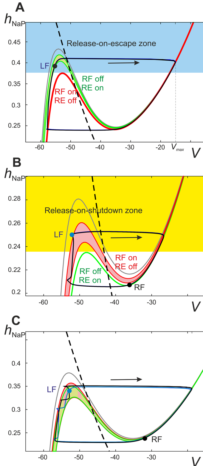
Fig 8. Fast-slow decomposition of the model dynamics when the inhibitory V_{0D} pathways are deleted. Projection of the phase portrait of the model onto the (V, h_{NaP}) plane at \alpha < X_6 . Sample positions, or image points, of flexor centers are depicted by the black (RF) and blue (LF) circles. A. Input from the right extensor center (RE) to the left flexor centers (LF) is represented as a sleeve of nullclines ranging from the maximal RE
