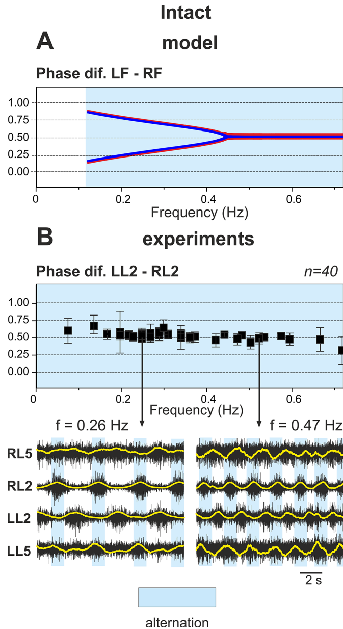
Fig 11. Phase-vs.-frequency bifurcation diagram for the intact model: Comparison with experimental data. A. The phase-vs.-frequency bifurcation diagram showing the dependence of phase difference between LF and RF on the oscillation frequency (transformed from “Phase dif. LF-RF” diagram in Fig 3B). For frequencies greater than 0.45 Hz the model demonstrated symmetric left-right alternation of flexor activity with \Delta\phi = 0.5 . For lower frequencies the flexors exhibited coupled alternation (see legend to Fig 3B and the text for details). B. The phase-vs.-frequency diagram summarizing experimental data from spinal cord preparations of wild type mice based on recordings from left (LL2) and right (RL2) lumbar roots. In this diagram, each square represents the mean phase difference between activities recorded from LL2 and RL2 in each preparation ( n = 40 ); error bars in each square indicate the standard deviation. Examples of two experimental recordings from RL5, RL2, LL2 and LL5 roots (raw recordings—black, and rectified—yellow) are shown at the bottom (vertical arrows indicate correspondence to the particular points in the upper diagram). Phase differences in all experiments remain close to 0.5 signifying alternating flexor behavior (details of recordings, measurements and processing can be found in [37]).
