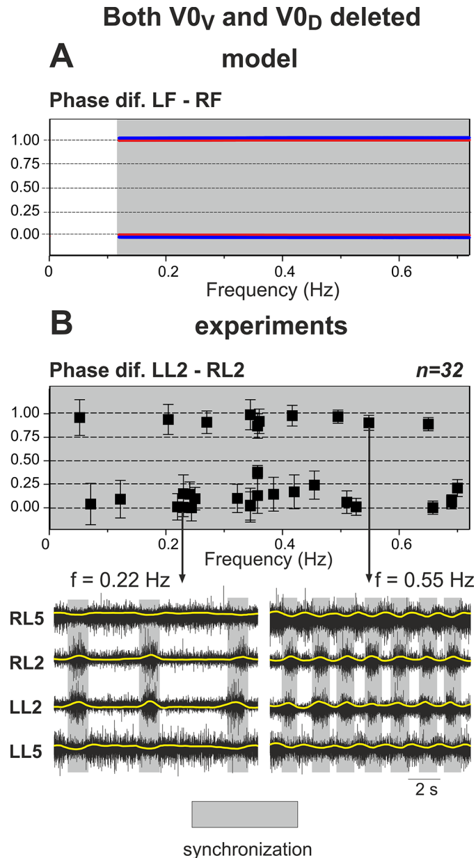
Fig 12. Phase-vs.-frequency bifurcation diagram for the model with both V0 pathways deleted: Comparison with experimental data. A. The phase-vs.-frequency bifurcation diagram for the model with both V0 pathways deleted (transformed from “Phase dif. LF-RF” diagram in Fig 4B). For all frequencies perfect left-right synchronization (hopping) is observed ( \Delta\phi = 0 or 1). B. The phase-vs.-frequency diagram summarizing experimental data from spinal cord preparations of knockout mice with deleted V0 commissural interneurons based on recordings from left (LL2) and right (RL2) lumbar roots. As in Fig 11B, each square represents the mean phase difference between LL2 and RL2 activities in each preparation ( n = 32 ). Examples of two experimental recordings from RL5, RL2, LL2 and LL5 roots (raw recordings—black, and rectified—yellow) are shown at the bottom (vertical arrows indicate correspondence to the particular points in the upper diagram). Phase difference remains close to 0 or 1 signifying synchronous flexor behavior. Reproduced from Talpalar et al. [37], Fig 2C and 2D.
