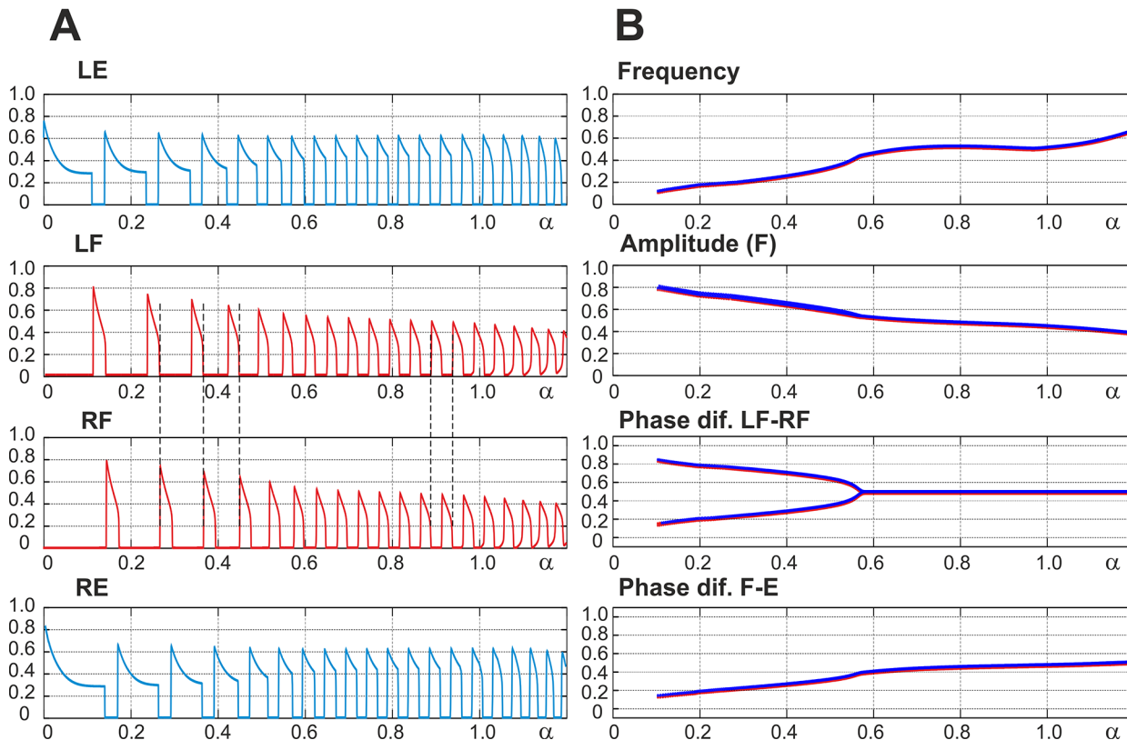
Fig 3. Performance of the intact model. A. Changes in the output activity of the four centers with increasing neuronal excitation ( \alpha ). LE and RE indicate left and right extensor centers, respectively; LF and RF indicate left and right flexor centers. For low values of \alpha ( \alpha < 0.55 ) RF activates upon LF shutdown (see vertical dashed lines). Due to asymmetry of flexor and extensor phase duration at low values of \alpha there is a part of each step cycle when both flexor centers are inactive and hence both extensor centers are active. \alpha was changed linearly in time from \alpha = 0 at t = 0 to \alpha = 1.2 at t = 120 s. B. Bifurcation diagrams for different dynamical characteristics. From top to bottom: Frequency —frequency of bursts in Hz; Amplitude (F) —flexor center amplitude (maximum output activity of flexor center); Phase dif. LF-RF —phase difference between left and right flexor centers; Phase dif. F-E —phase difference between ipsilateral flexor and the extensor centers. When \alpha increases there is an increase in frequency (mostly concerned with shortening of extensor phase) as well as a decrease in the amplitude of each flexor center burst (see also LF and RF panels on the left). For relatively high values of excitation ( \alpha > 0.55 ) the phase difference between flexor centers is exactly 0.5. This means that the RF activates exactly one half-period after the LF . At lower values of \alpha two distinct regimes exist: the first has a phase difference between flexor centers less than 0.5 (lower branch) which corresponds to the activation pattern shown in A ( LF leads, RF activates on LF 's shutdown, then a pause until LF activates again) and the second regime has a phase difference greater than 0.5 (upper branch) when RF activates first and LF activates on RF 's shutdown (not shown on A ). Note that in all diagrams in B , \alpha was changed in both directions, first forward from 0 to 1.2 and then backward from 1.2 to 0. However, in all diagrams in Fig 3B, the graphs for forward (red) and backward (blue on the top) changes of \alpha overlapped. In summary, the intact model demonstrates left-right alternating activity at all levels of excitation (all values of \alpha ).
