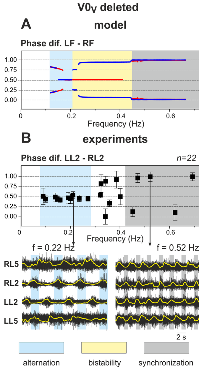
Fig 13. Phase-vs.-frequency bifurcation diagram for the model with V0 v pathways deleted: Comparison with experimental data. A. The phase-vs.-frequency bifurcation diagram for the model with only V0 v pathways deleted (transformed from “Phase dif. LF-RF” diagram in Fig 5B). Alternating behavior occurs at low frequencies and hopping at high frequencies with an area of bistability separating the two (between approximately 0.2 and 0.42 Hz). B. The phase-vs.-frequency diagram summarizing experimental data from spinal cord preparations of knockout mice with selective removal of V0 v commissural interneurons based on recording from left (LL2) and right (RL2) lumbar roots. As in Figs 10B and 11B, each square represents the mean phase difference between LL2 and RL2 activities in each preparation ( n = 22). Examples of two experimental recordings from RL5, RL2, LL2 and LL5 roots (raw recordings—black, and rectified—yellow) are shown at the bottom (vertical arrows indicate correspondence to the particular point in the upper diagram). Phase difference is near 0.5 at low frequencies and close to 0 or 1 at high frequencies signifying alternating and synchronous flexor behavior, respectively. For the intermediate frequencies (from about 0.3 to 0.42 Hz) phase differences are widely distributed and intermittently synchronized behavior is observed. Reproduced from Talpalar et al. [37], Fig 4D and 4E.
