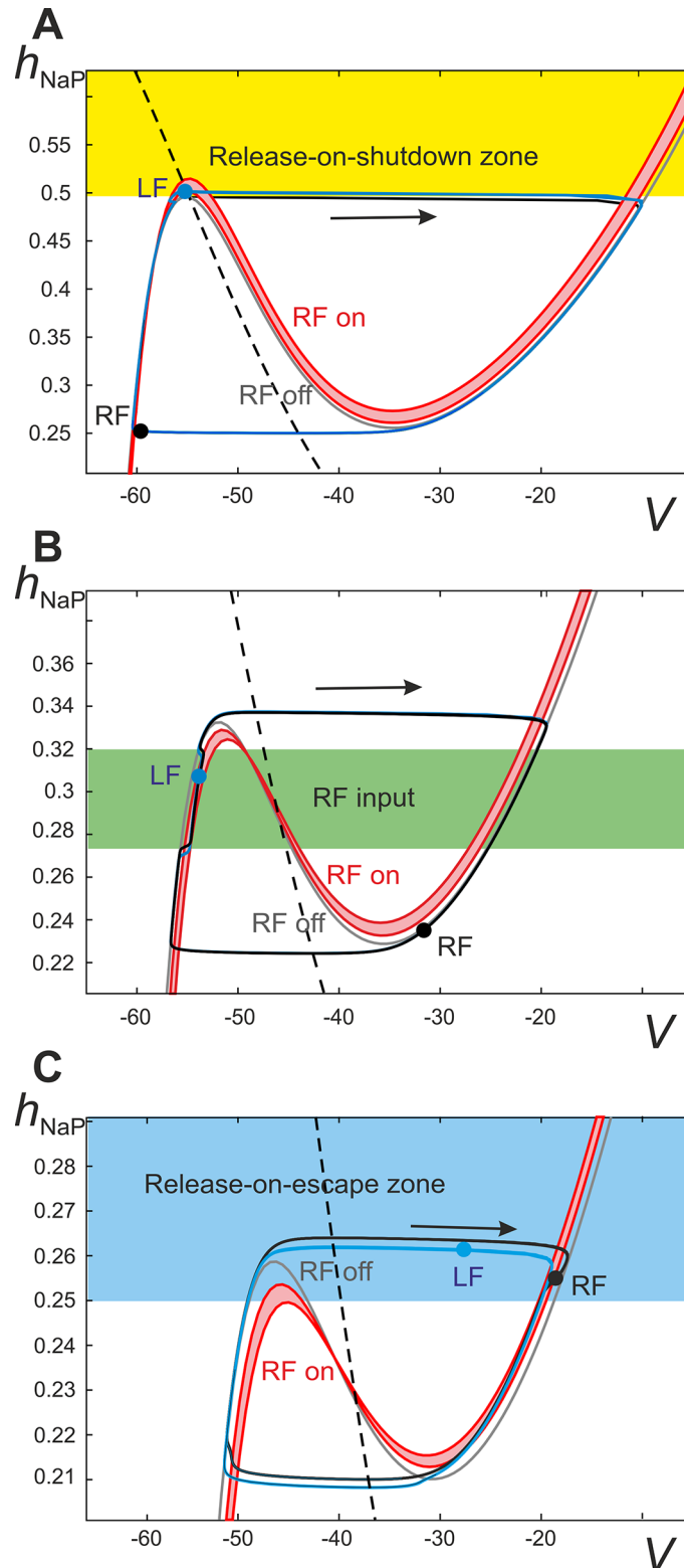
Fig 6. Fast-slow decomposition of the model dynamics when the V_{0v} excitatory pathways are deleted. The trajectories of left and right flexor centers (LF and RF) are projected onto the (V, h_{NaP}) plane (blue and black curves, respectively). The red nullcline band (RF on) depicts the range of input received by the left flexor center from the right flexor center during the activity period of the latter. Due to a gradual decrease of
