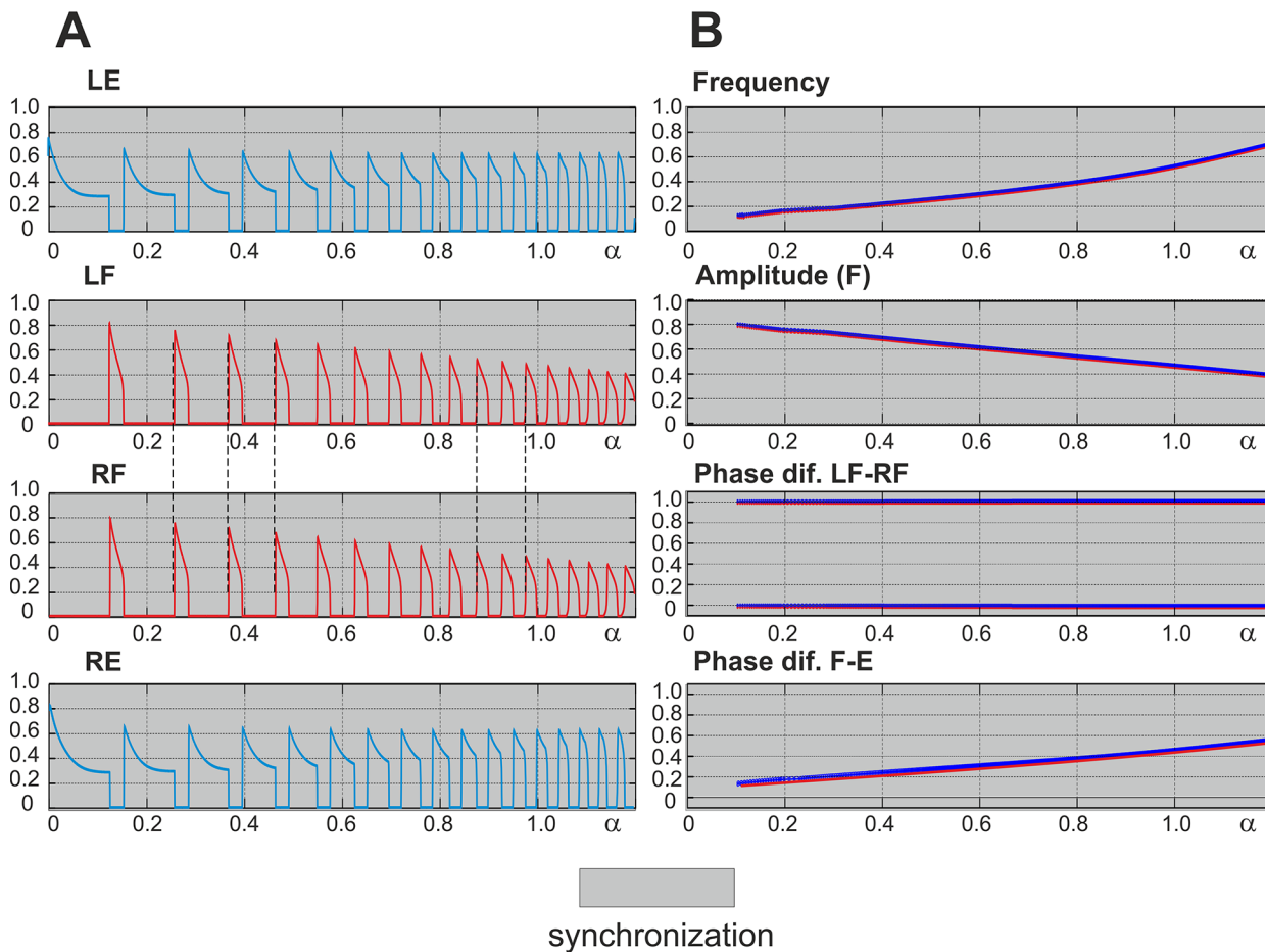
Fig 4. Performance of the model with both V0 pathways removed. A. Changes in the activity of the four centers with increasing neuronal excitation ( \alpha ). Mutual excitation between LF and RF maintains left-right synchronized behavior as indicated by the dashed lines. B. Bifurcation diagrams. Frequency and amplitude of flexor center oscillations change similarly to the intact case (see Fig 3 for comparison). The phase difference between LF and RF is 0 or 1, indicating perfect left-right synchronization for all values of \alpha . Other details and explanations can be found in the legend to Fig 3. As in the intact case, \alpha was changed in both directions, first forward from 0 to 1.2 (red) and then backward from 1.2 to 0 (blue on the top), but graphs for forward and backward changes of \alpha overlap. In summary, when both V0 pathways are removed, the model exhibits left-right synchronized “hopping” behavior at all levels of excitation (all values of \alpha ).
