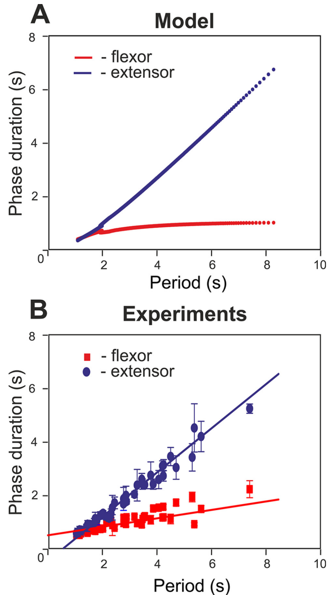
Fig 10. Changing the flexor and extensor phase durations with oscillation period. A. Graphs were built for the intact model by varying excitation ( \alpha ). B. Flexor and extensor phase durations vs. step cycle period from wild-type mice spinal cord preparations ( n = 11 ). The step cycle period was varied by application of NMDA. Data were obtained from the recording originally published in [37].
