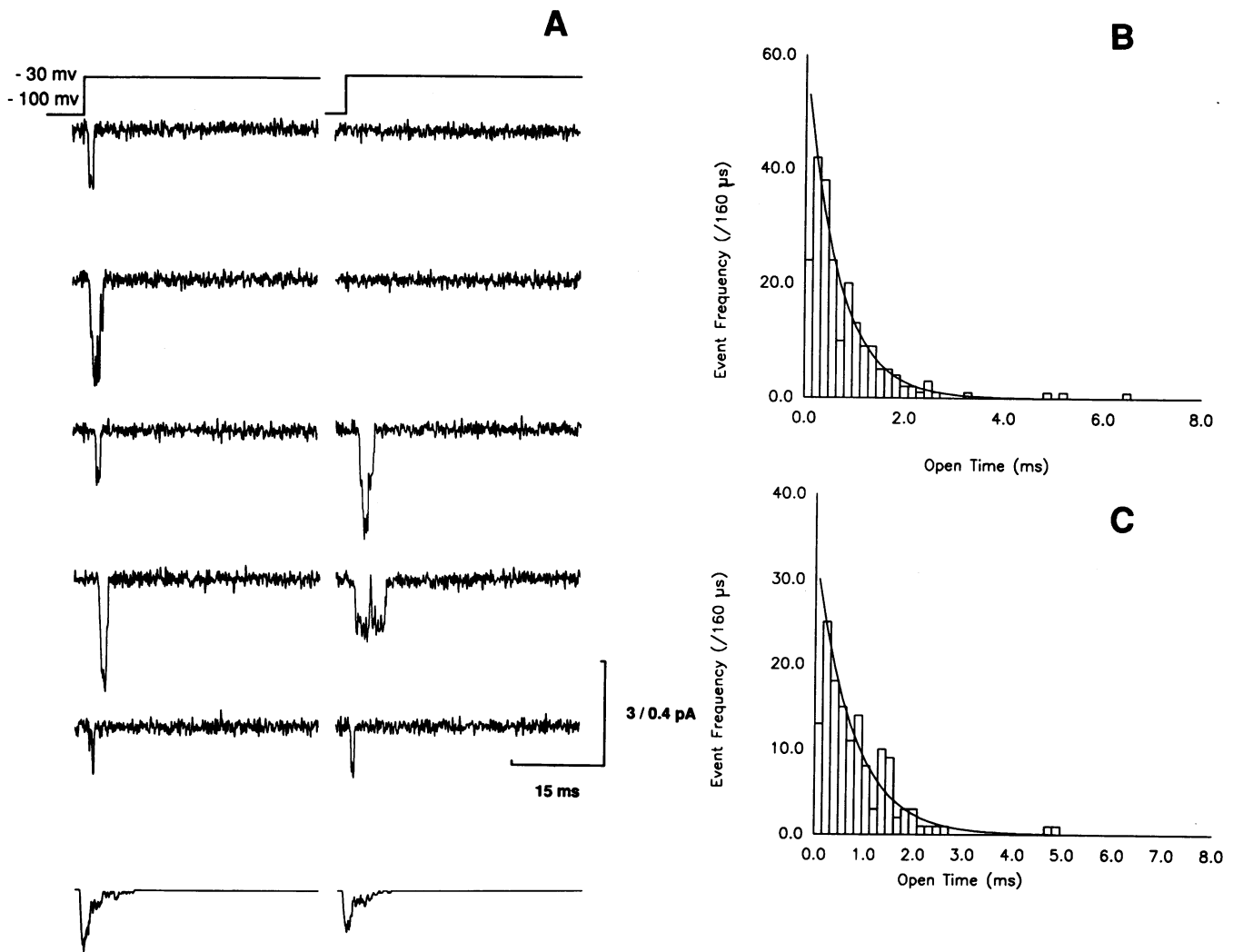
Figure 10. Single-channel current with conditioning and test pulses during exposure to 80 \mu\text{M} lidocaine. The holding potential was -100\text{ mV} and the test potential -30\text{ mV} . The average current, shown on the lowest trace, was decreased during the test pulse. The mean closing rate was 1.5/ms and 1.3/ms for the conditioning and test pulses, respectively. Current and time calibrations of 3 and 0.4 pA shown in the insert refer to the individual and average current traces, respectively.
