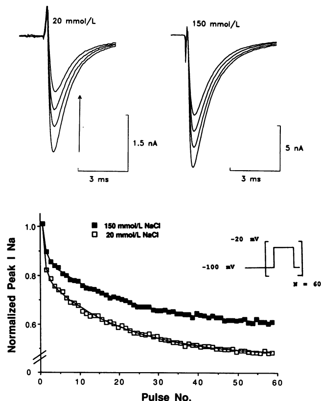
Figure 5. Use-dependent block during exposure to 100 \mu\text{M} disopyramide. The current traces show sodium channel current in response to a train of 50-ms pulses from a holding potential of -100 \text{ mV} to a test potential of -20 \text{ mV} . In the lower portion of the figure, the normalized peak Na current is plotted as a function of the order of the pulses in the train. The continuous lines represent double-exponential fits to the data points. For [\text{Na}]_o of 20 mM, the time constants for block development were 0.67 and 19.8 pulses; for [\text{Na}]_o of 150 mM 0.79 and 20.6 pulses. L, liter.
