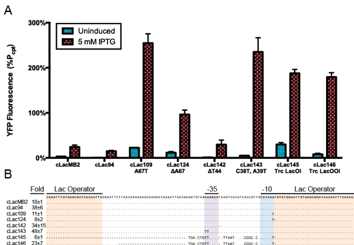
Figure 6. Diagram and induction levels for IPTG inducible promoters. (A) Expression of induced and uninduced IPTG inducible promoters relative to P cppt . With the exception of the P cppt control, all strains contain lacI expressed by P MB2 . All cLac### strains have the additional W220F mutation in lacI while cLacMB2 contains wildtype lacI . Error bars represent standard deviation of biological replicates ( n = 3 ) (B) List of IPTG inducible promoters with fold induction potential (fold change between 0 and 5 mM IPTG) and sequence comparison. The lac operators are highlighted in yellow, the -35 sequence is highlighted in purple, and the -10 sequence is highlighted in green.
