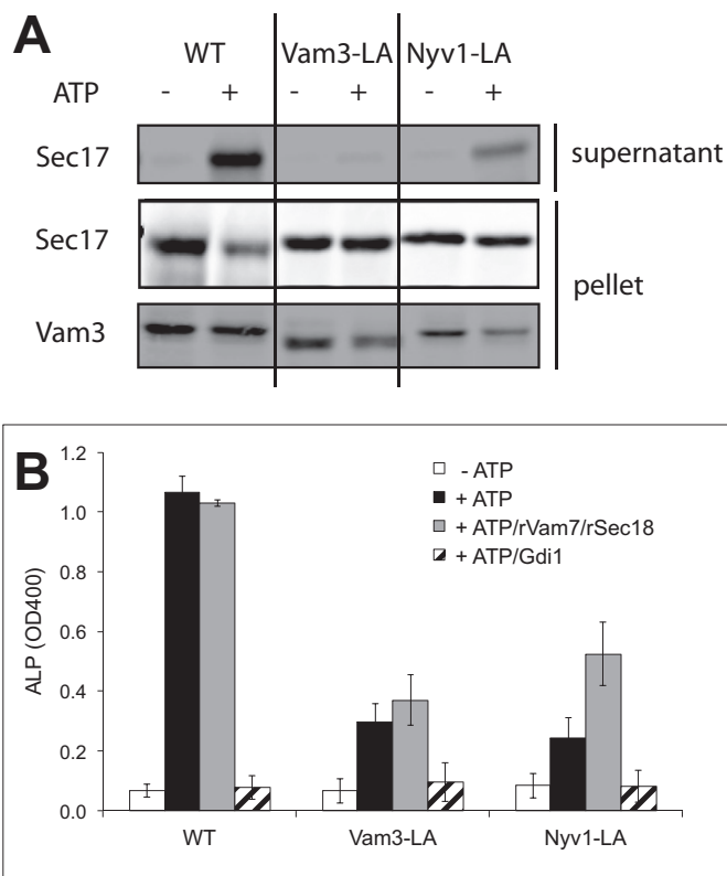
FIGURE 3. SNARE activation in Vam3-LA and Nyv1-LA mutants. A , vacuoles with lipid-anchored Vam3 and Nyv1 were incubated in fusion reactions in the presence or absence of ATP. The release of Sec17 was assayed by pelleting the vacuoles and blotting for the released protein. B , content mixing was analyzed with vacuoles bearing Vam3-LA and Nyv1-LA or the respective WT proteins. Fusion reactions had been incubated in the presence or absence of rVam7 (1.2 \mu M) and rSec18 (60 nM). Means \pm S.D. are shown for three independent experiments.
