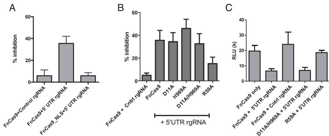
Fig. 3. Molecular requirements for Fncas9-mediated HCV inhibition. (A) Huh-7.5 cells were transfected with Fncas9 \pm NLS, the 5' UTR-targeting rgRNA, and HCV. At 72 h, viral luciferase was quantified and the percent inhibition compared with the nontargeting rgRNA is displayed ( n = 8 ; data compiled from three independent experiments). (B) Experiments were performed as above, using alanine point mutants in the RuvC domain (D11A), HNH domain (H969A), the double mutant (D11A/H969A), or the ARM (R59A) ( n = 8 ; data compiled from three independent experiments). (C) Rabbit reticulocyte lysate in vitro translation assays of HCV luciferase were performed using the indicated Cas9 and RNAs and viral luciferase measured ( n = 4 ; data are representative of four experiments).
