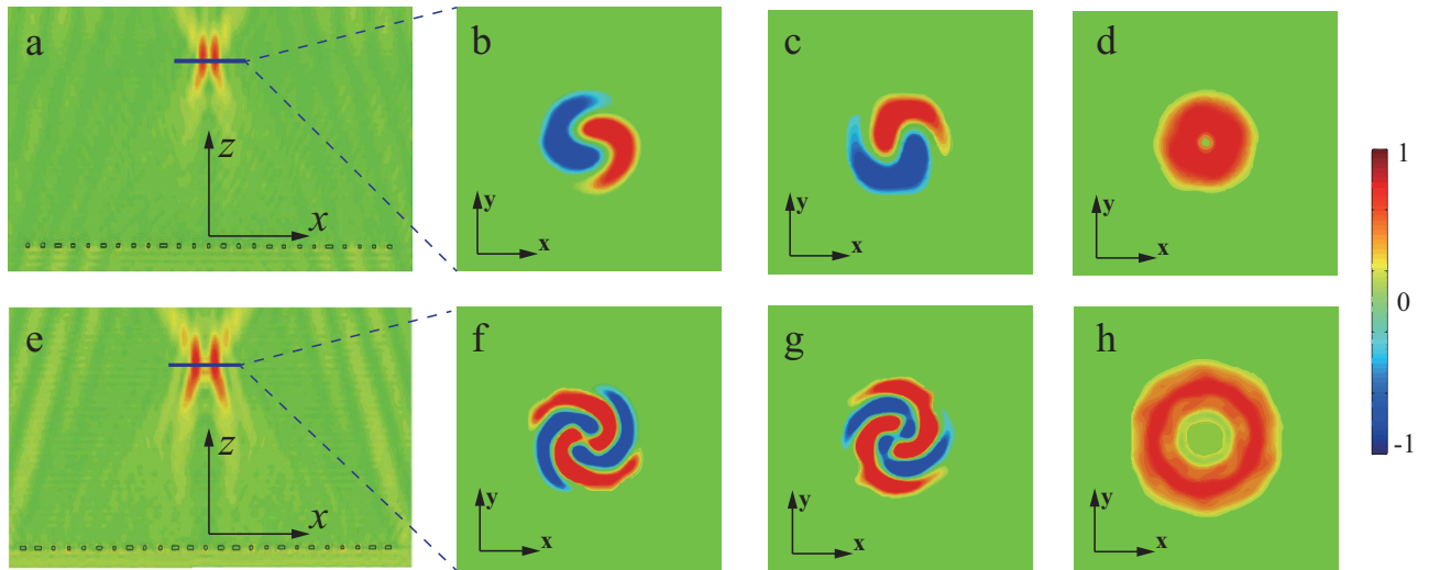
Figure 3. Simulated electric field distribution of the generated optical vortex beam for l = 1, 2 . (a) The energy intensity of outgoing electric field of converted OAM light with l = 1 in xoz plane. (b) x - and (c) y -component of the instant radiated electric field in xy plane at the focus. (d) The energy intensity of the radiating electric field for optical vortex with topological charge l = 1 in xy plane. (e) The energy intensity of outgoing electric field in xoz plane of the OAM beam with topological charge l = 2 . (f)–(h) x -, y -components and the energy intensity of the generated focused optical vortex with topological charge of l = 2 in xy plane at the focus, respectively.
