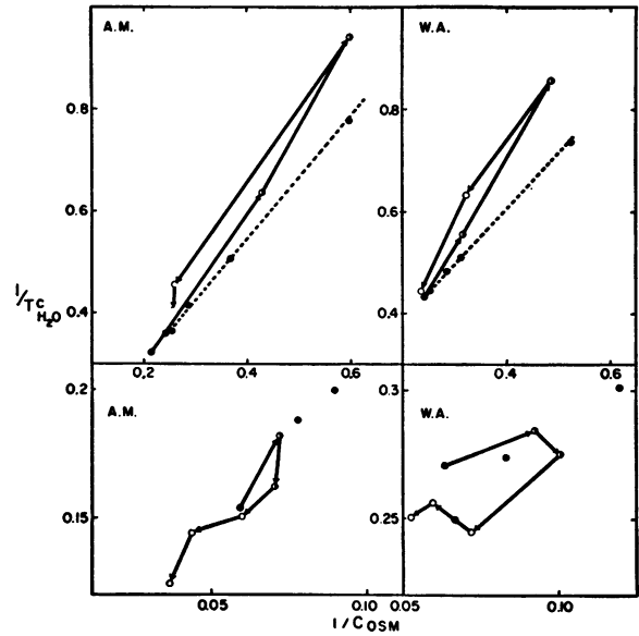
FIG. 2. THE RELATIONSHIP BETWEEN NET WATER REABSORPTION ( T^cH_2O ) AND OSMOLAL CLEARANCE ( C_{osm} ) EXPRESSED AS THE RECIPROCAL 1/T^cH_2O AND 1/C_{osm}
